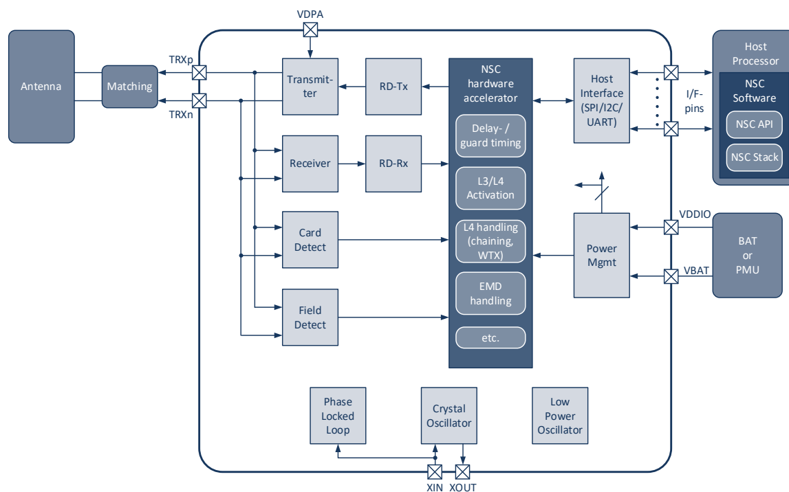
Figure 1: Block Diagram
