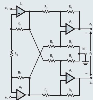
DIFFERENTIAL OUTPUT INSTRUMENTATION AMPLIFIER
