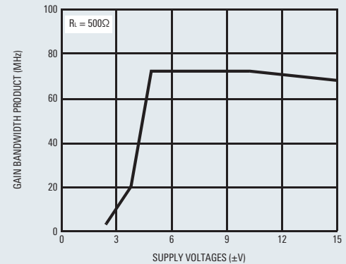
GAIN BANDWIDTH PRODUCT vs SUPPLY
