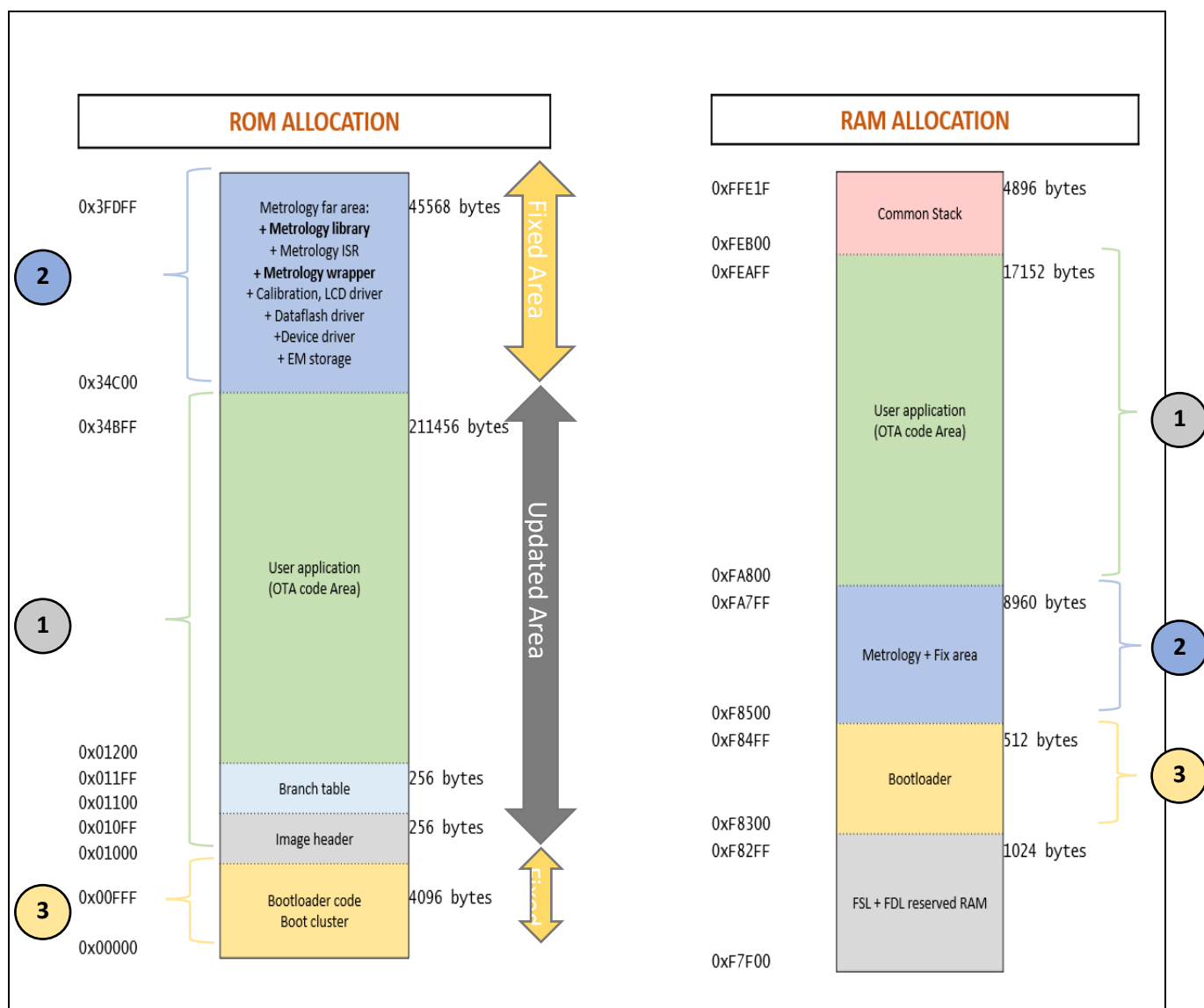
Figure 4-2 Memory allocation for Fast FOTA and Continuous Metrology FOTA
