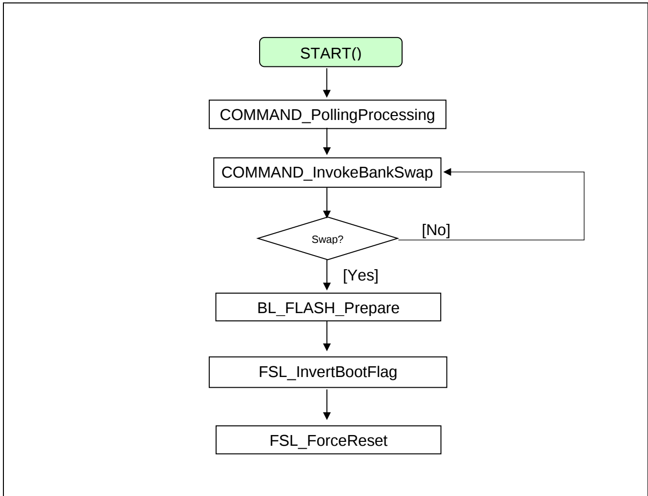
Figure 5-1 Usage of Fast FOTA API
