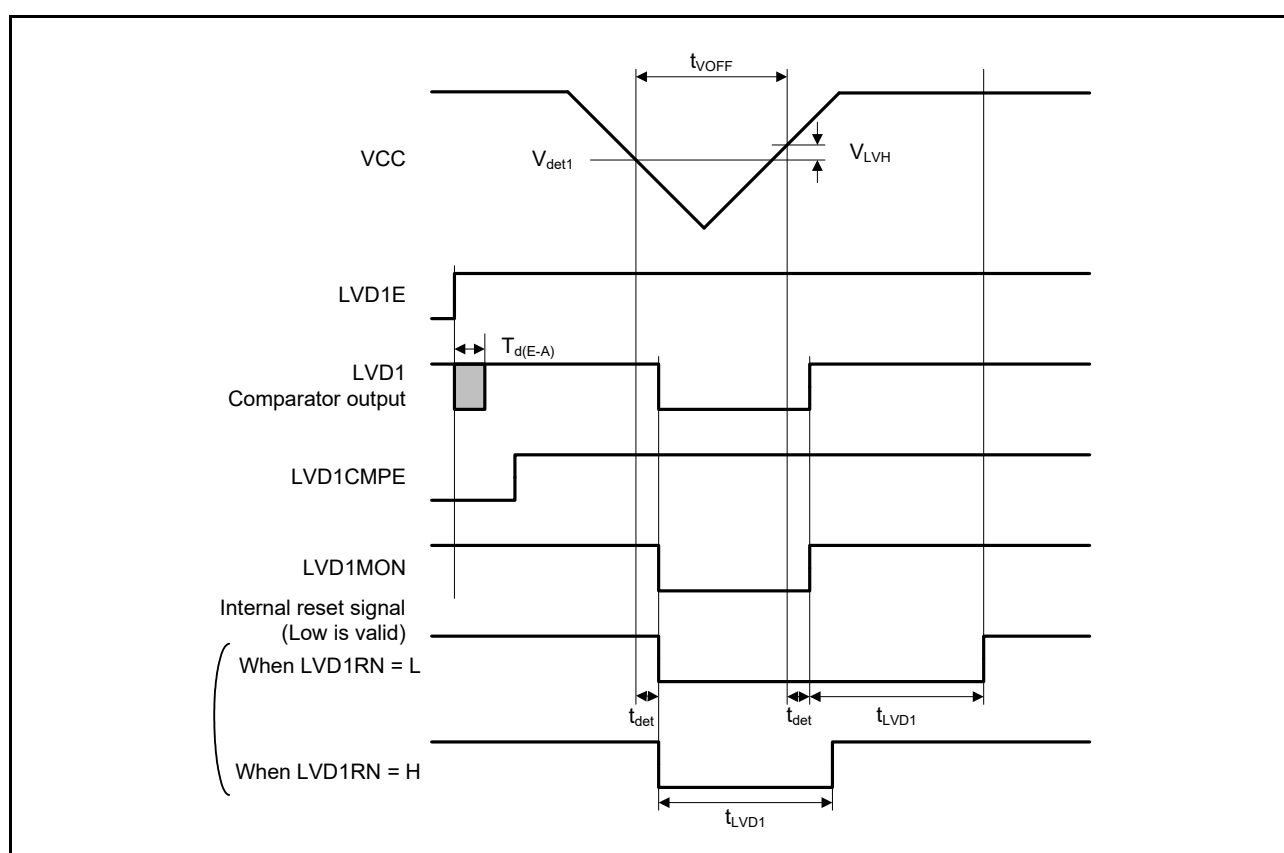
Figure 2.80 Voltage Detection Circuit Timing (V det1 )
