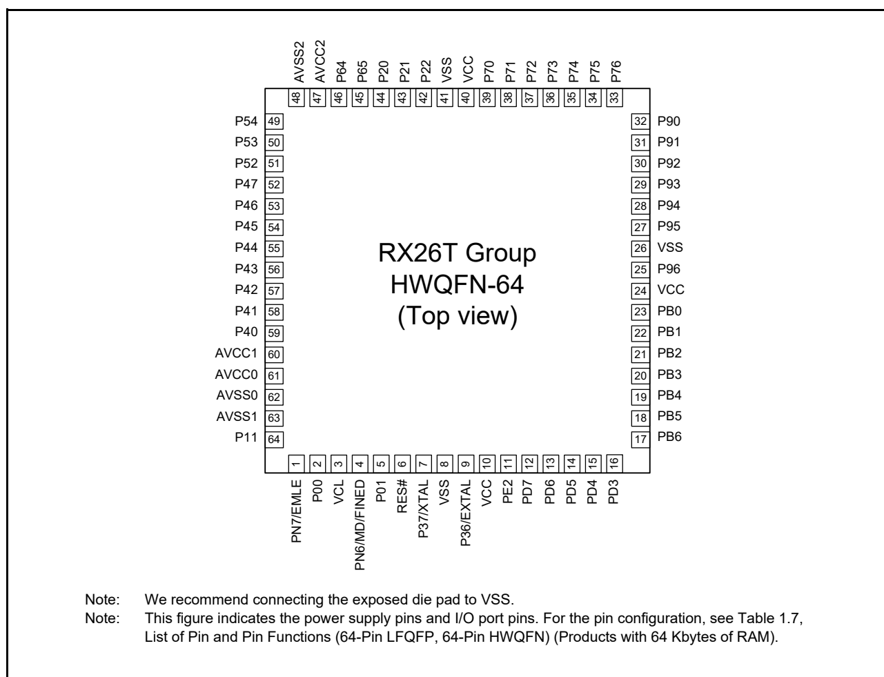
Figure 1.8 Pin Assignment (64-pin HWQFN)
