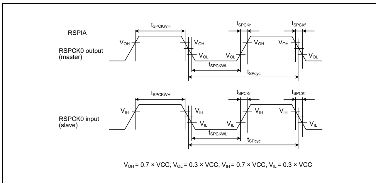
Figure 2.59 RSPIA Clock Timing
