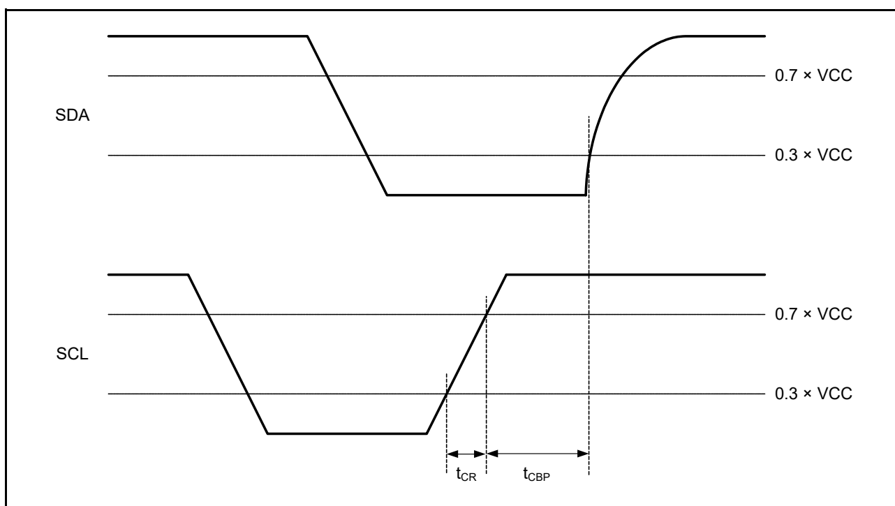
Figure 2.70 RI3C Stop Condition Timing
