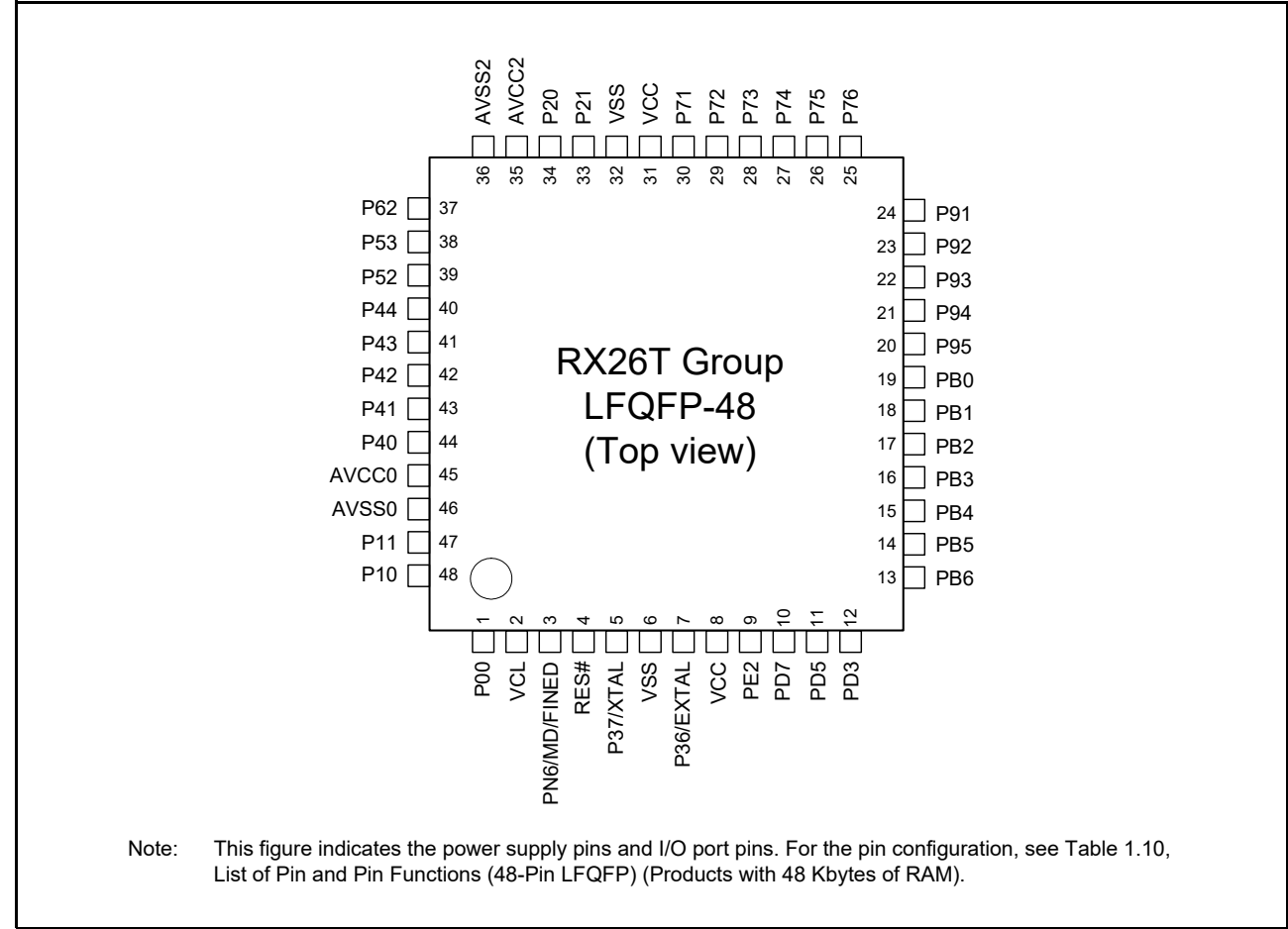
Figure 1.10 Pin Assignment (48-pin LFQFP) (Products with 48 Kbytes of RAM)
