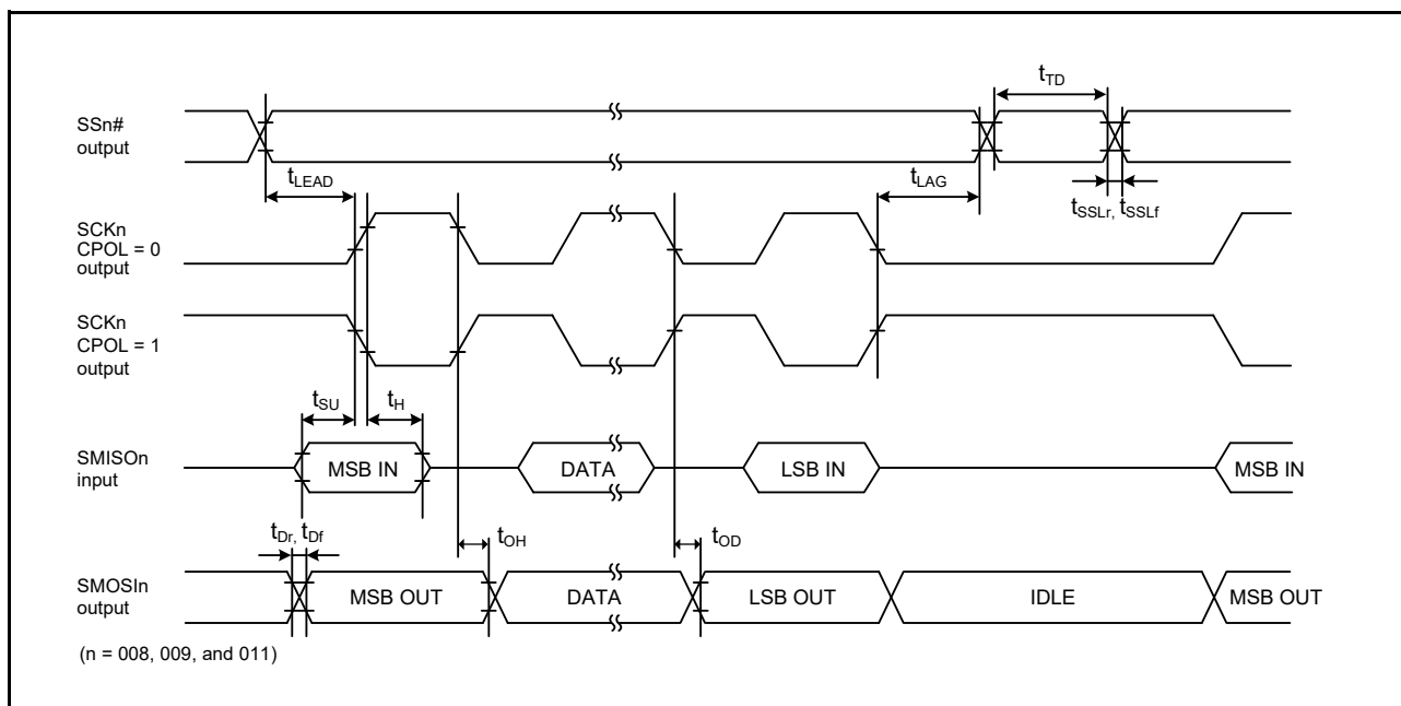
Figure 2.48 Simple SPI Timing (Master, CPHA = 0)
