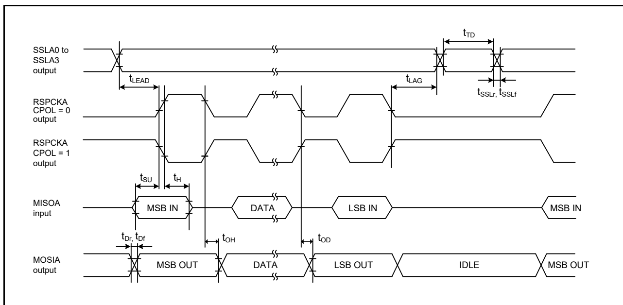
Figure 2.53 RSPI Timing (Master, CPHA = 0) (Bit Rate: PCLKA Division Ratio Set to a Value Other Than 1/2)
