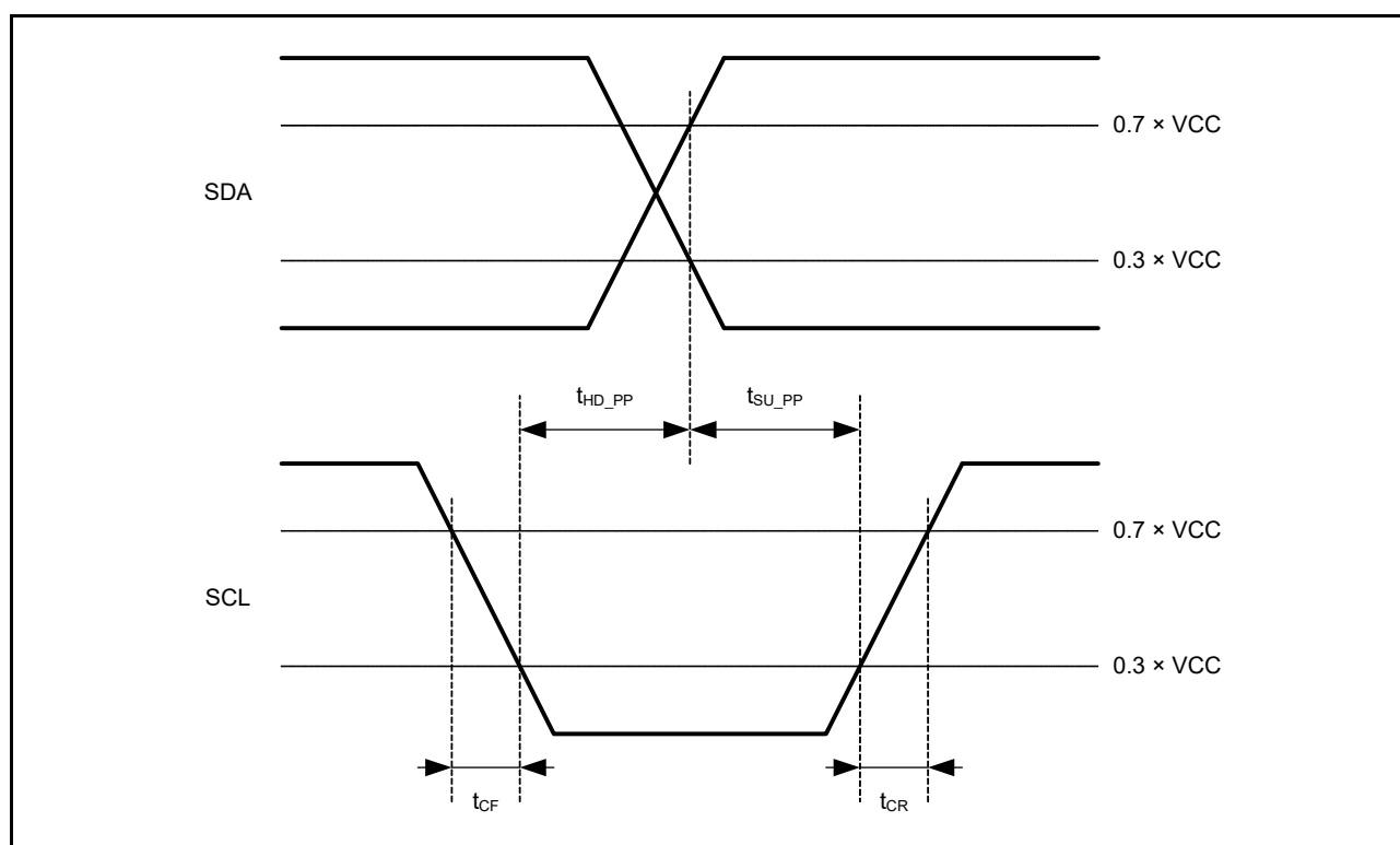
Figure 2.74 R13C Bus Controller Output Timing
