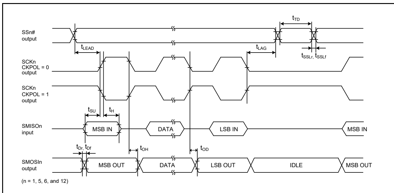
Figure 2.40 Simple SPI Timing (Master, CKPH = 1)
