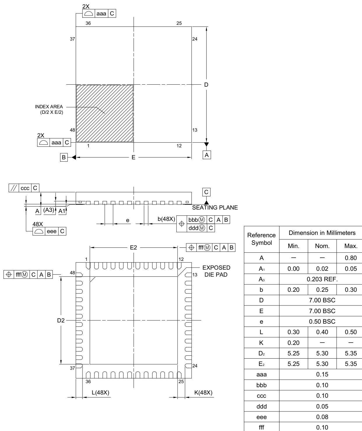
Figure F 48-Pin HWQFN (PWQN0048KC-A)
