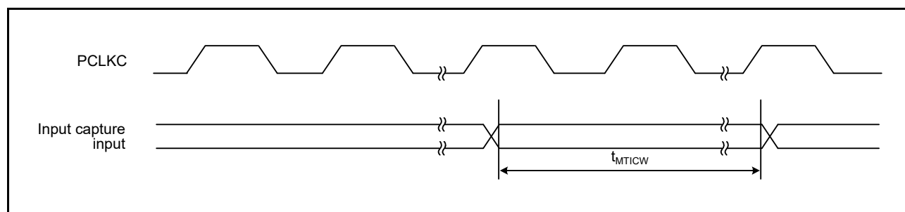
Figure 2.16 MTU Input Capture Input Timing
