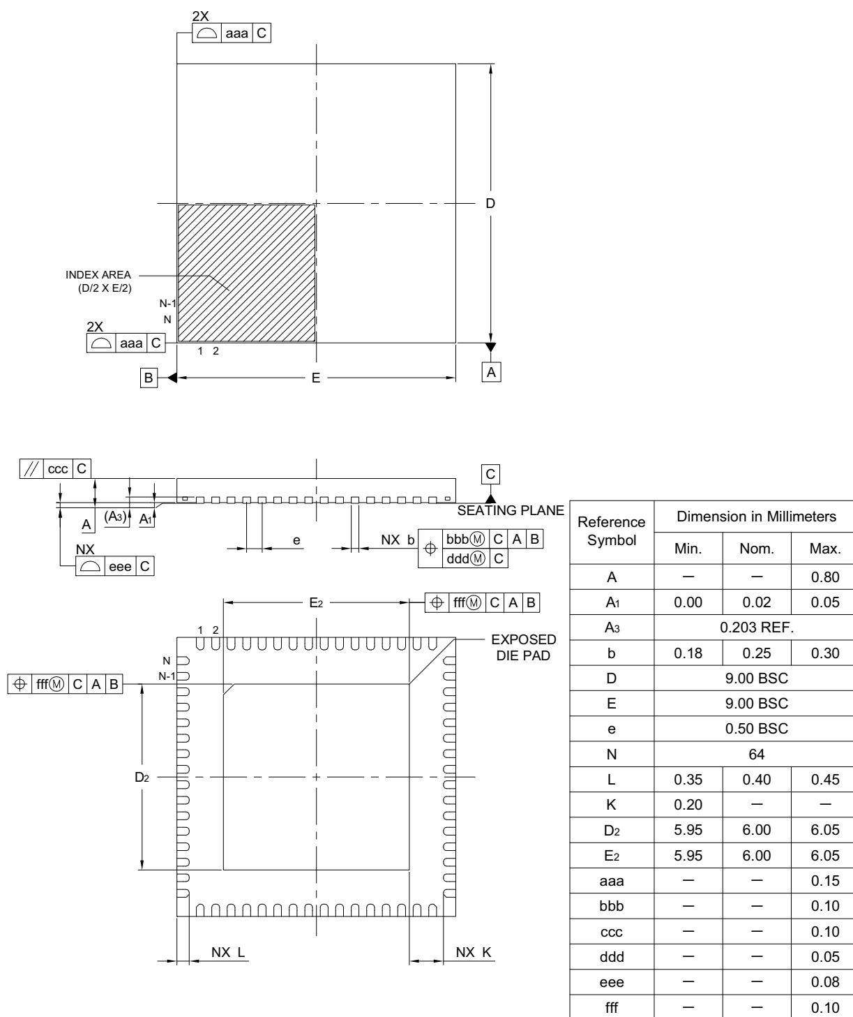
Figure D 64-Pin HWQFN (PWQN0064KF-A)
