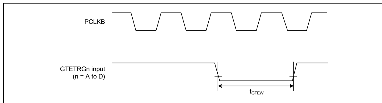
Figure 2.33 GPTW External Trigger Input Timing
