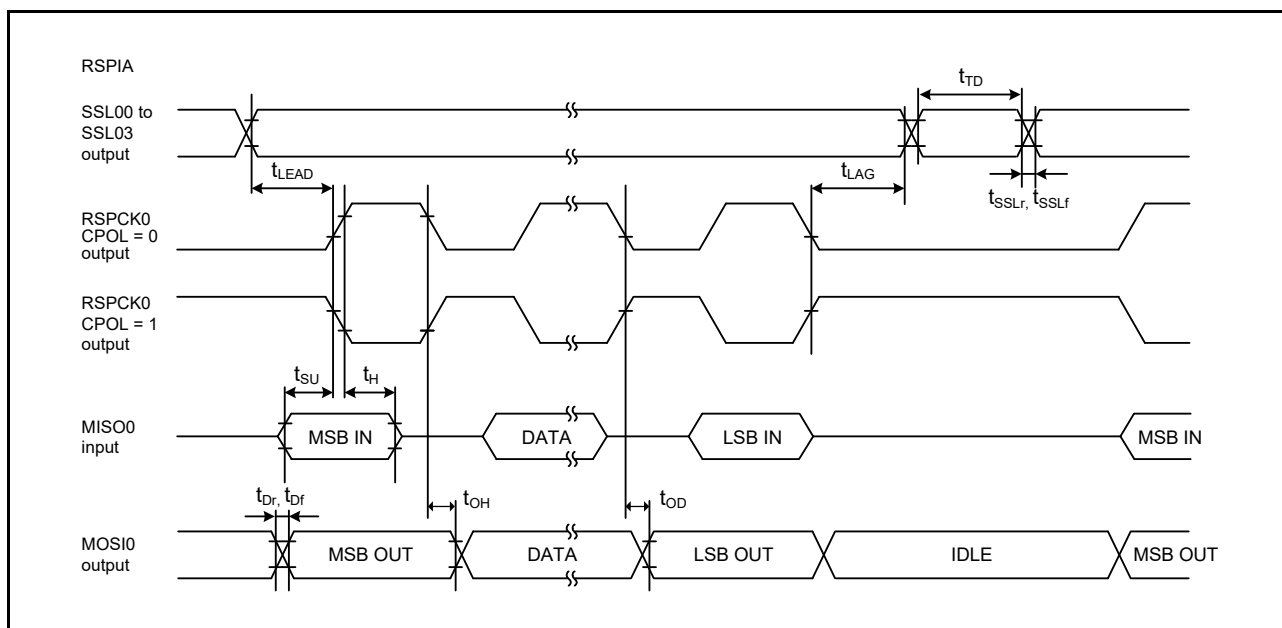
Figure 2.60 RSPIA Timing (Master, Motorola SPI, CPHA = 0)
