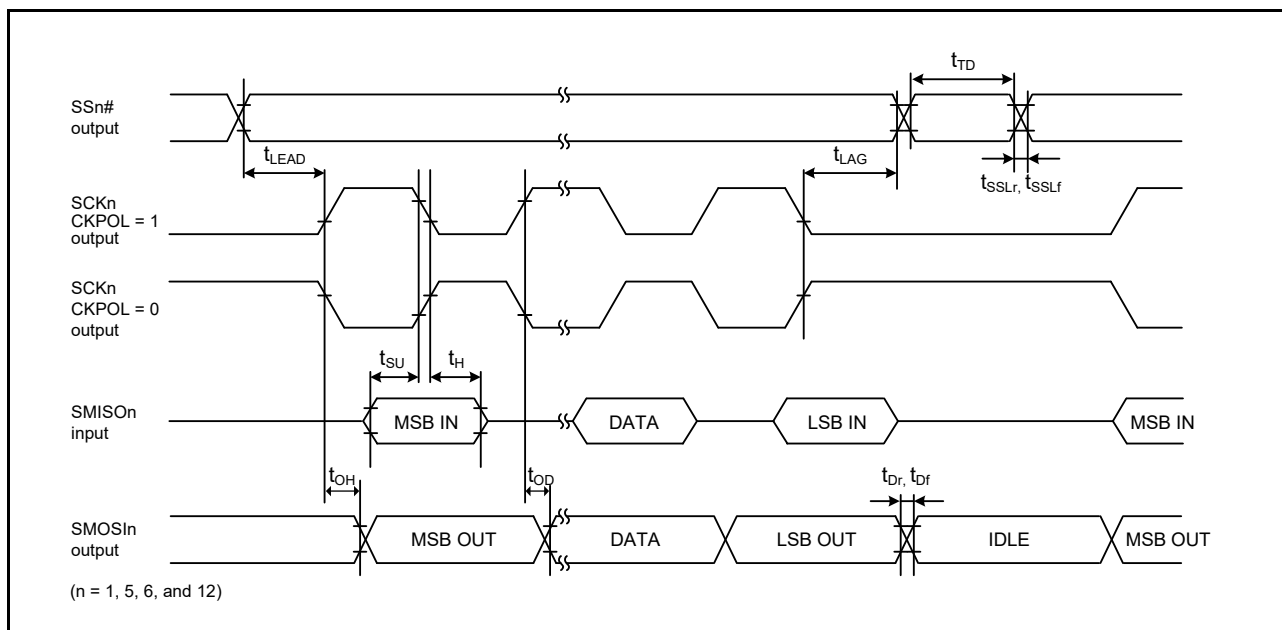
Figure 2.41 Simple SPI Timing (Master, CKPH = 0)
