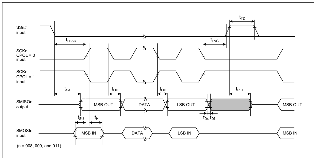
Figure 2.50 Simple SPI Timing (Slave, CPHA = 0)
