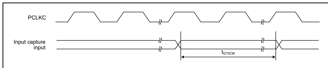
Figure 2.32 GPTW Input Capture Input Timing
