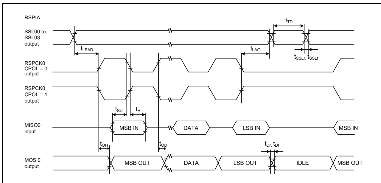
Figure 2.61 RSPIA Timing (Master, Motorola SPI, CPHA = 1)
