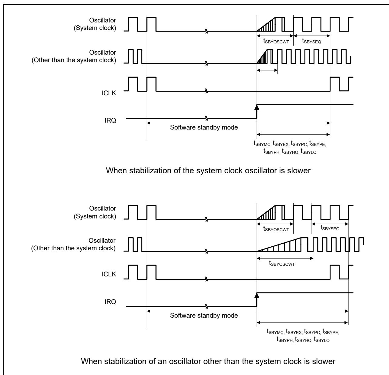
Figure 2.11 Software Standby Mode Cancellation Timing
