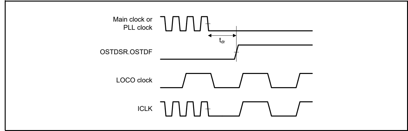
Figure 2.82 Oscillation Stop Detection Timing
