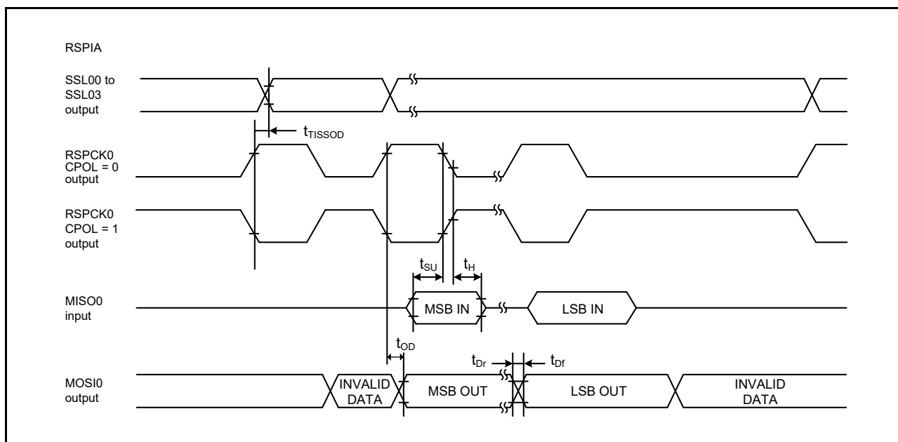
Figure 2.62 RSPIA Timing (Master, TI SSP)
