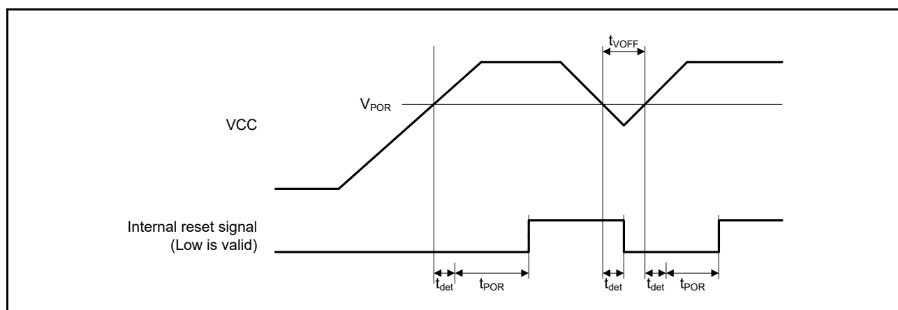
Figure 2.78 Power-on Reset Timing
