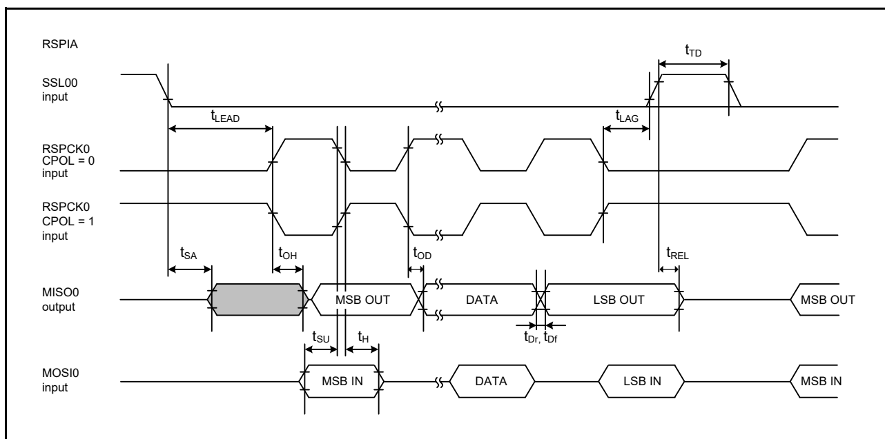
Figure 2.64 RSPIA Timing (Slave, Motorola SPI, CPHA = 1)
