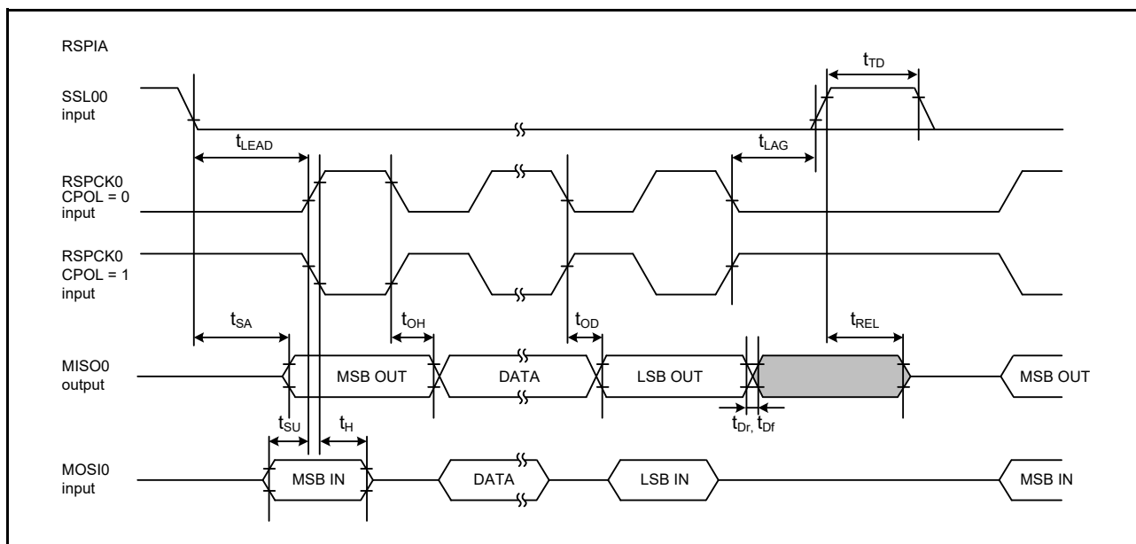
Figure 2.63 RSPIA Timing (Slave, Motorola SPI, CPHA = 0)
