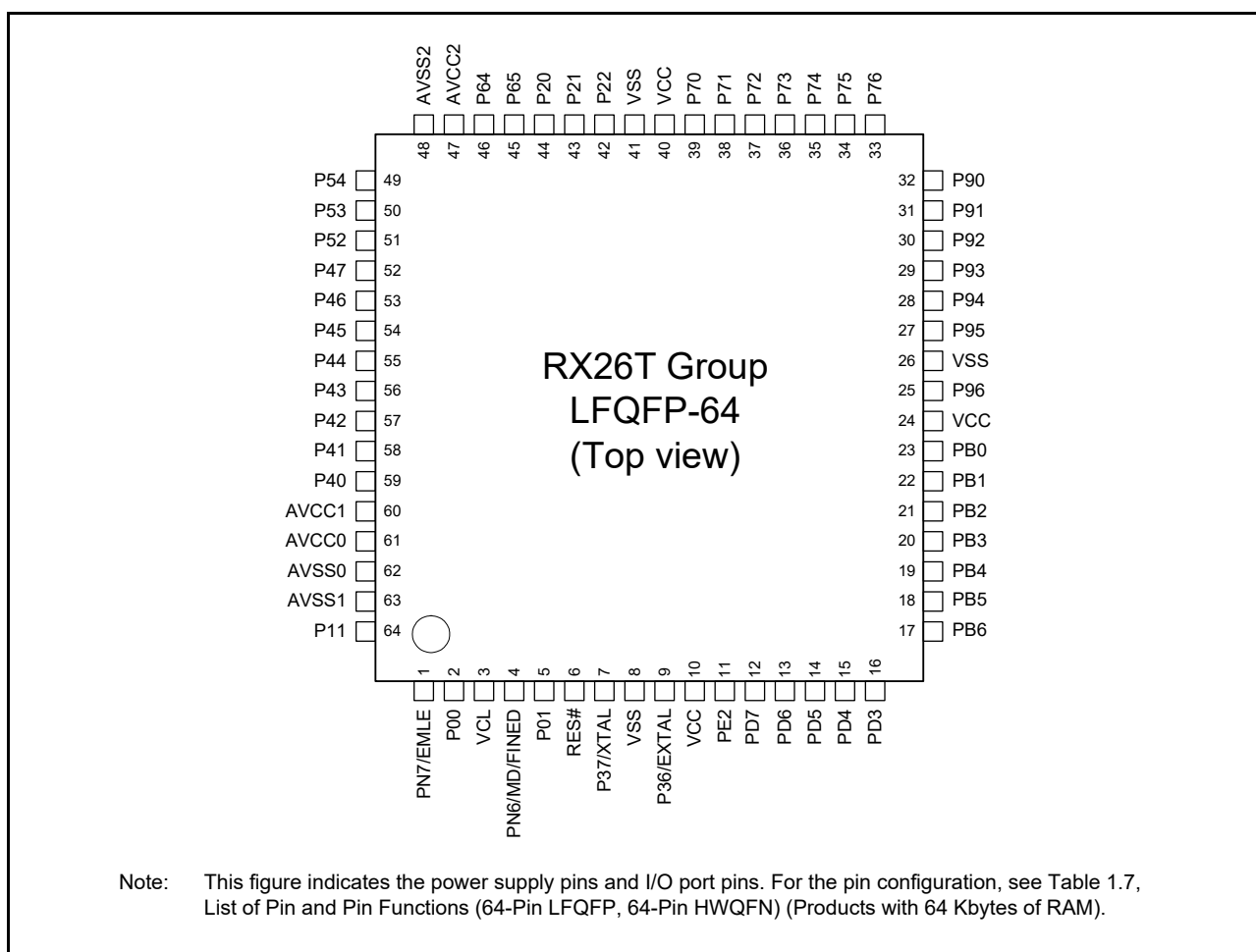
Figure 1.6 Pin Assignment (64-pin LFQFP) (Products with 64 Kbytes of RAM)
