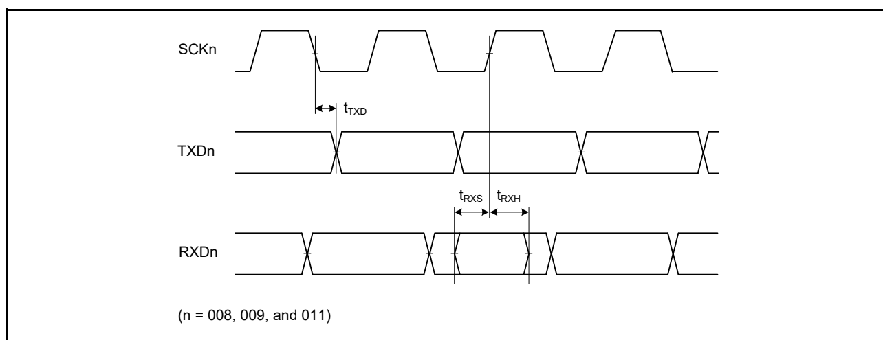
Figure 2.45 RSCI Input/Output Timing: Clock Synchronous Mode
