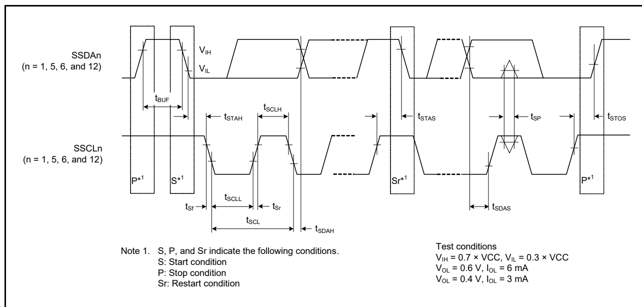
Figure 2.38 Simple IIC Bus Interface Input/Output Timing
