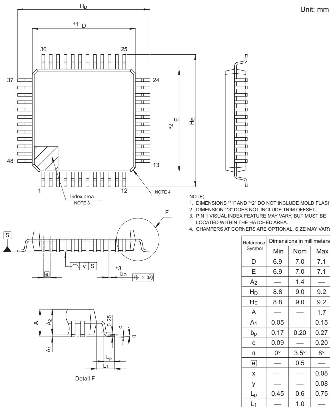
Figure E 48-Pin LFQFP (PLQP0048KB-B)
