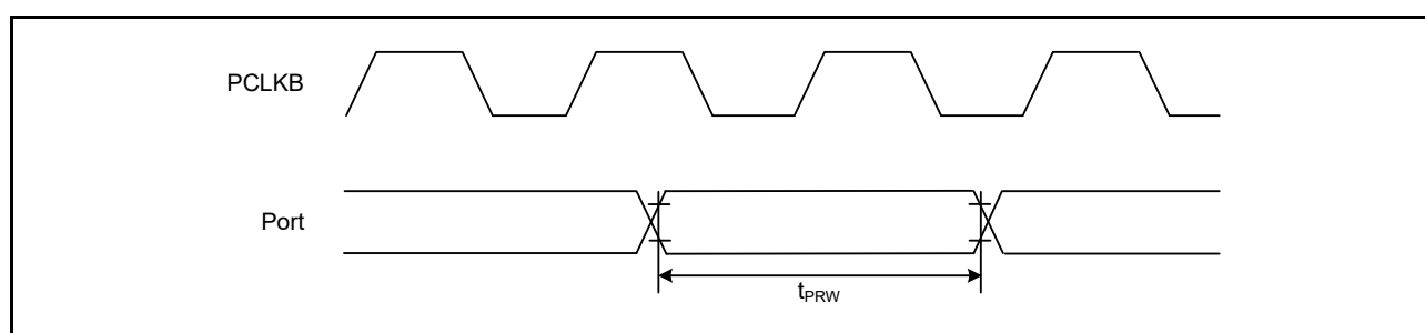
Figure 2.14 I/O Port Input Timing
