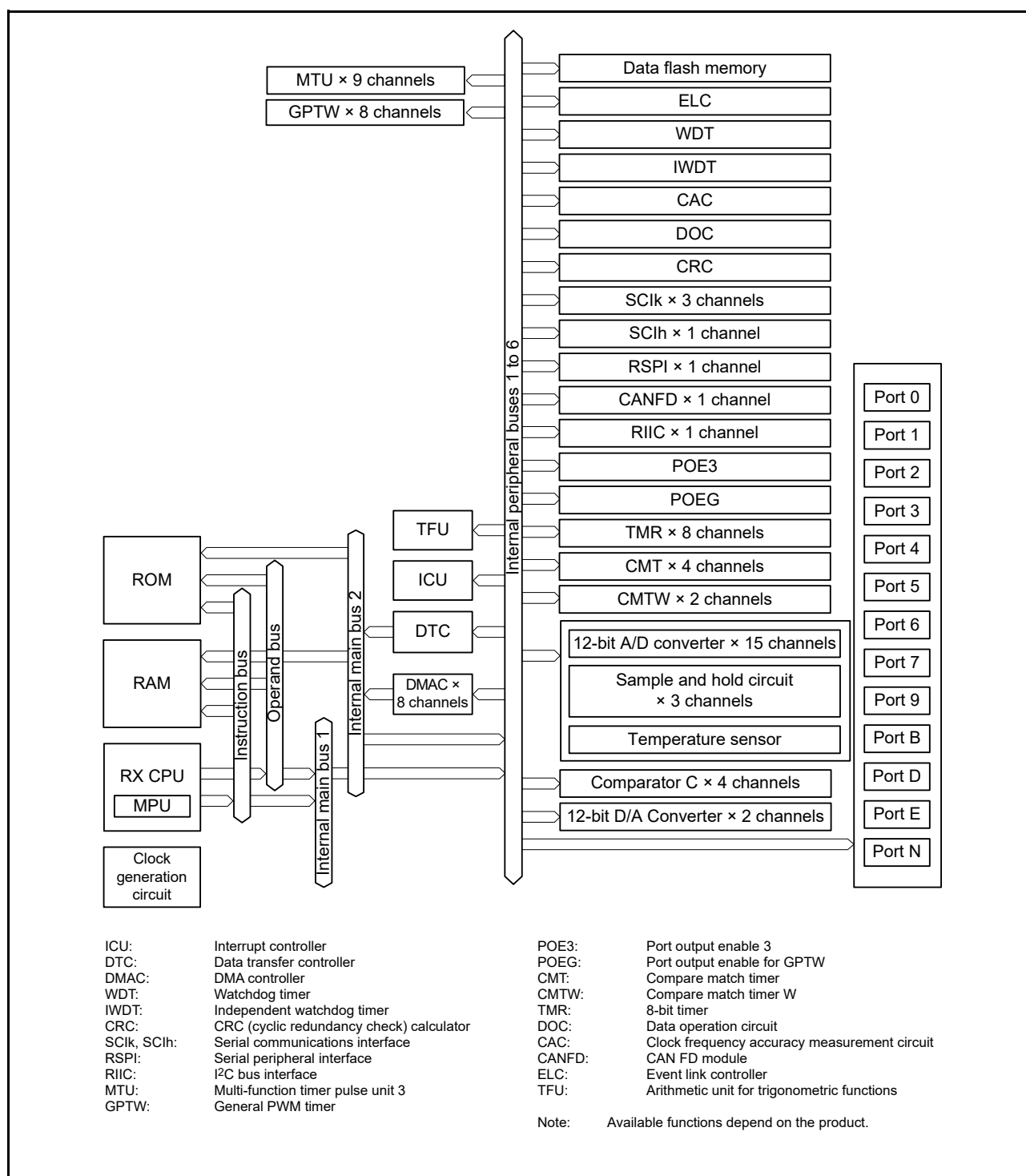
Figure 1.3 Block Diagram (Products with 48 Kbytes of RAM)
