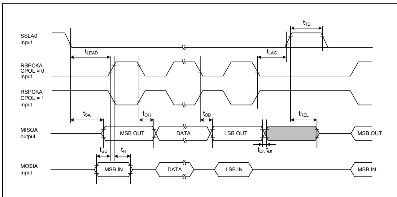
Figure 2.57 RSPI Timing (Slave, CPHA = 0)
