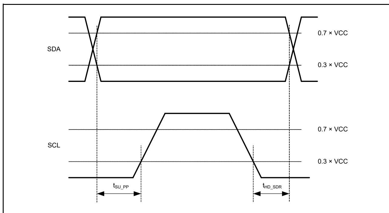
Figure 2.75 Controller SDR Timing
