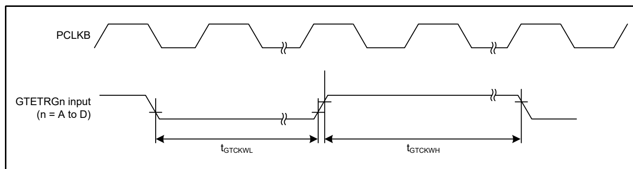
Figure 2.34 GPTW Clock Input Timing
