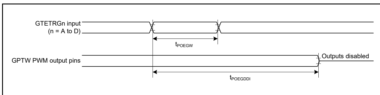
Figure 2.30 Output Disable Time for POEG in Direct Response to the Input Level Detection of the GTETR Gn pin
