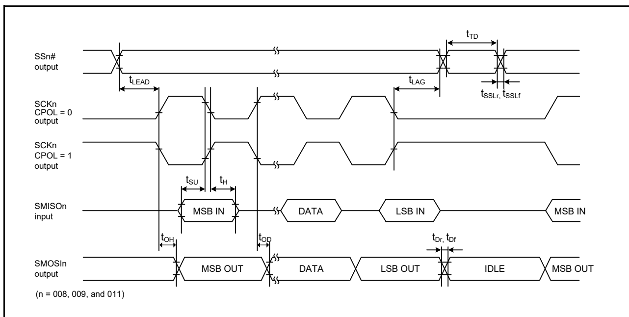
Figure 2.49 Simple SPI Timing (Master, CPHA = 1)
