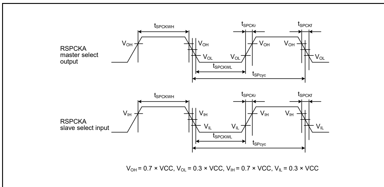
Figure 2.52 RSPCKA Clock Timing
