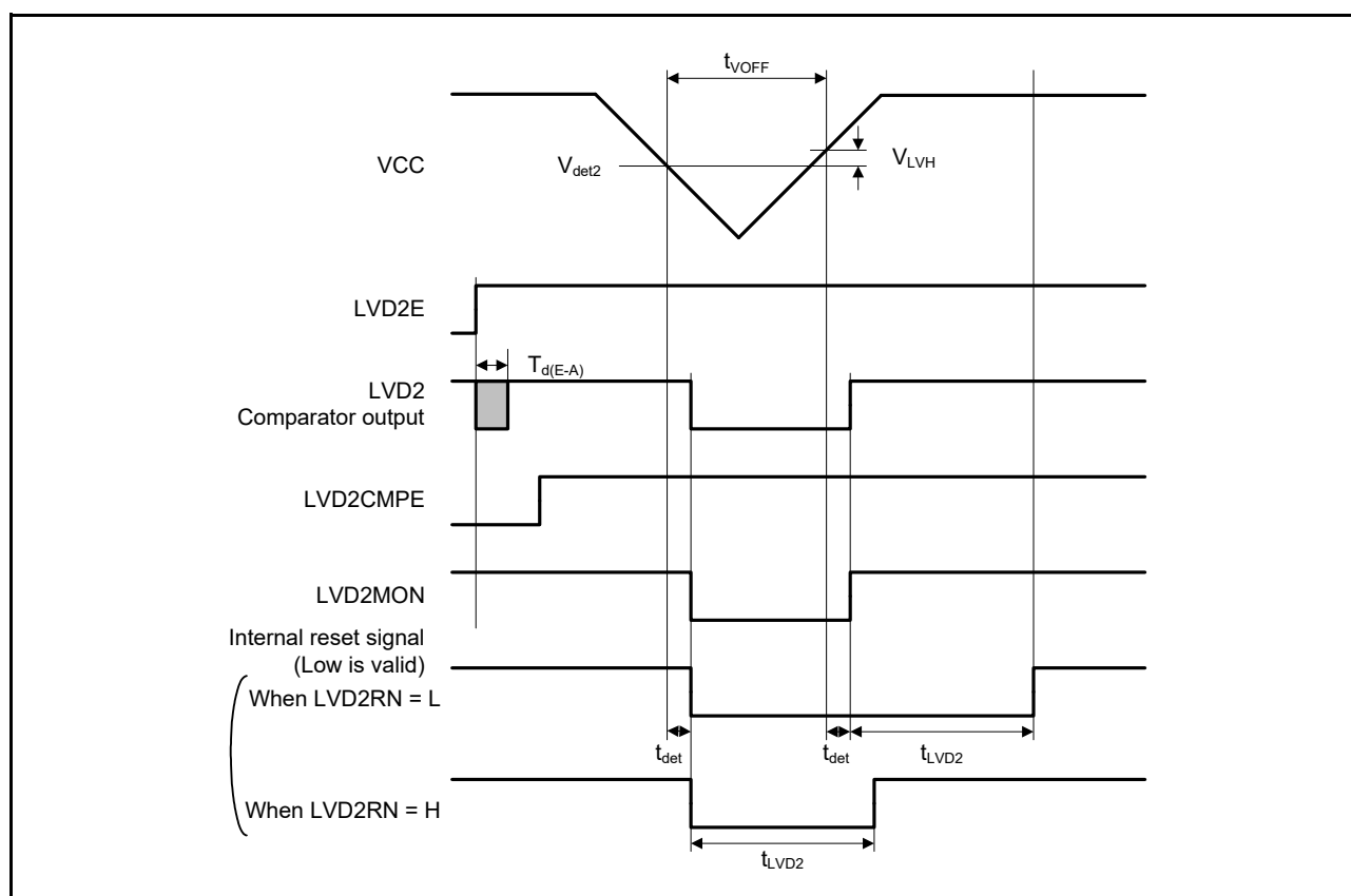
Figure 2.81 Voltage Detection Circuit Timing (V det2 )
