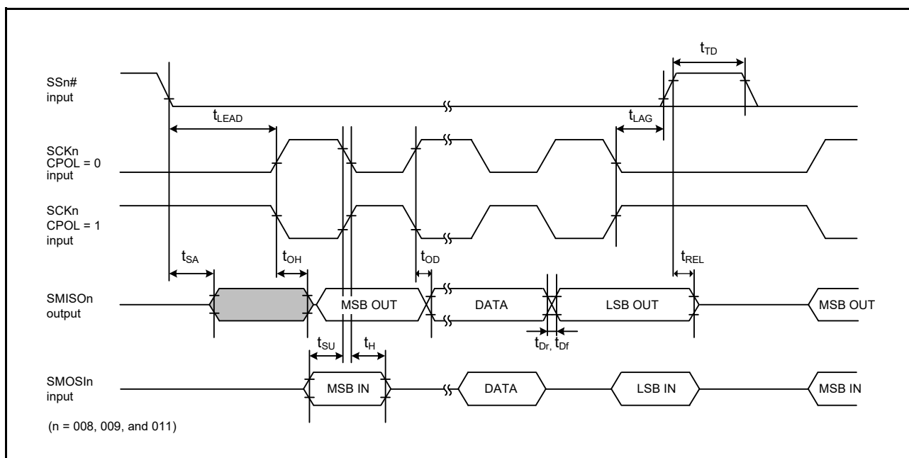
Figure 2.51 Simple SPI Timing (Slave, CPHA = 1)
