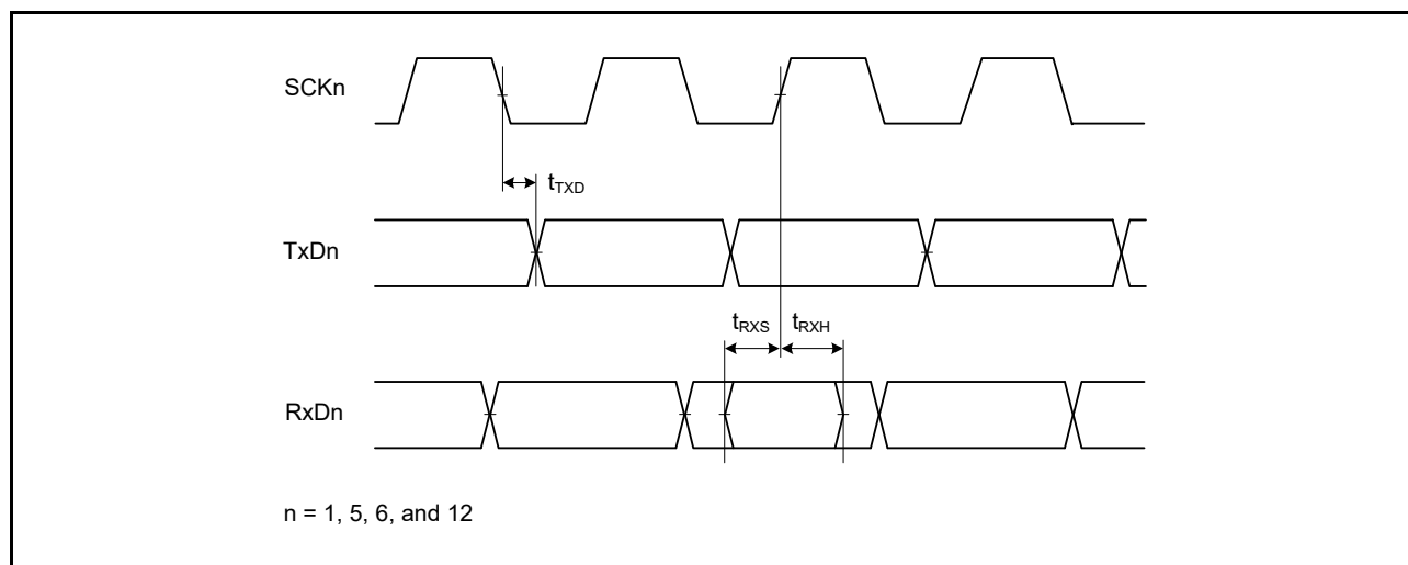
Figure 2.37 SCI Input/Output Timing: Clock Synchronous Mode
