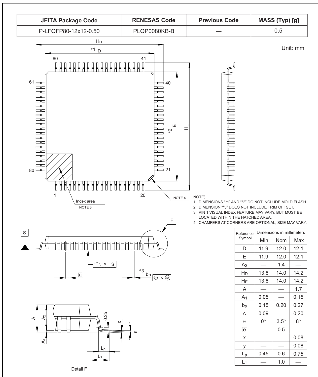
Figure B 80-Pin LFQFP (PLQP0080KB-B)
