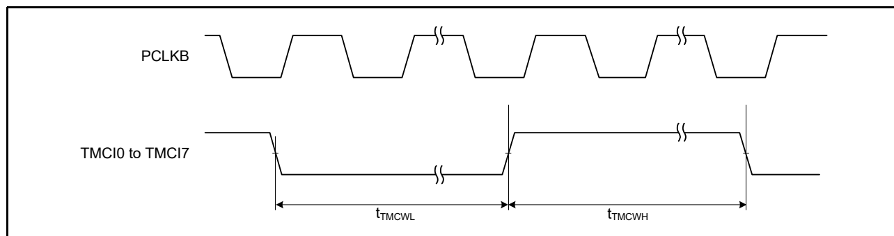
Figure 2.15 TMR Clock Input Timing
