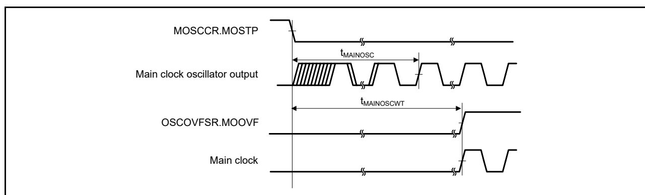
Figure 2.5 Main Clock Oscillation Start Timing
