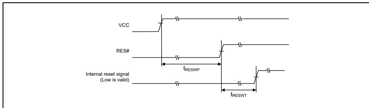
Figure 2.2 Reset Input Timing at Power-On
