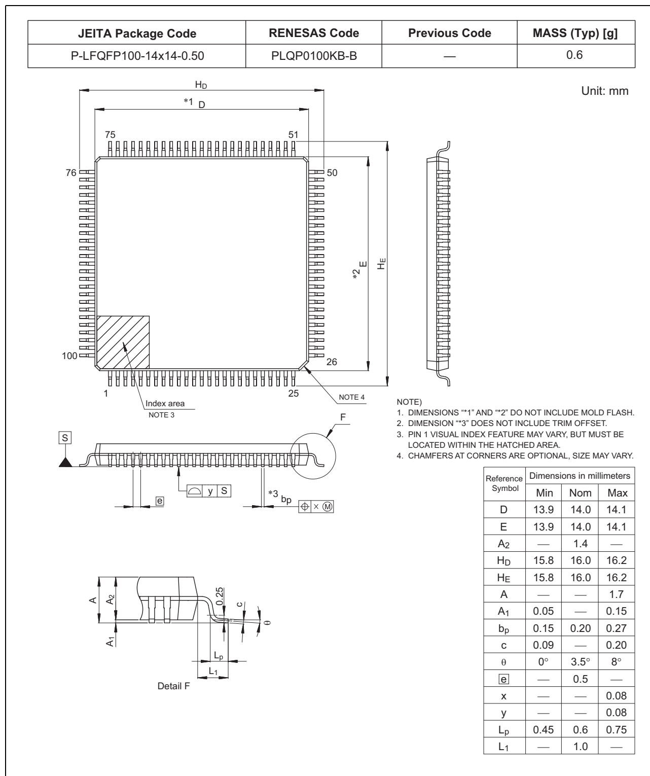
Figure A 100-Pin LFQFP (PLQP0100KB-B)
