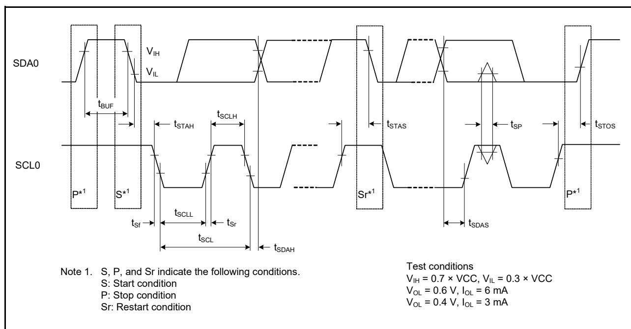
Figure 2.67 IIC Bus Interface Input/Output Timing
