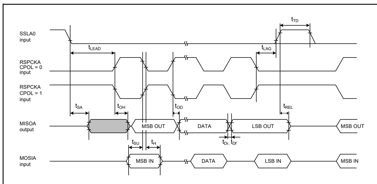
Figure 2.58 RSPi Timing (Slave, CPHA = 1)
