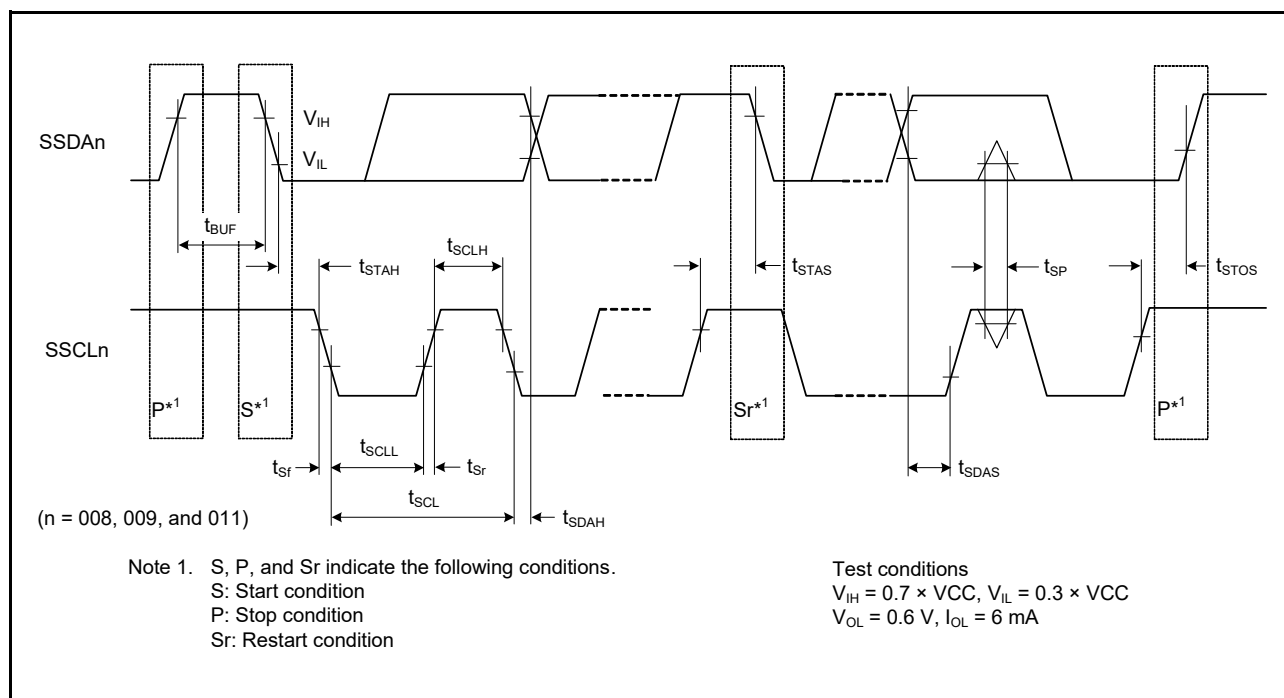
Figure 2.46 Simple IIC Bus Interface Input/Output Timing
