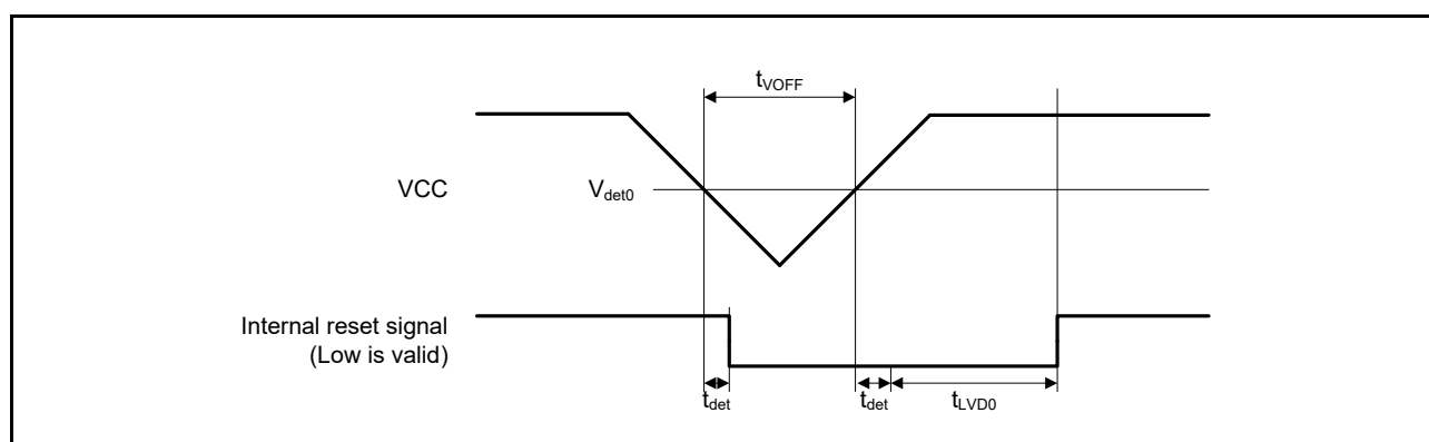
Figure 2.79 Voltage Detection Circuit Timing (V det0 )
