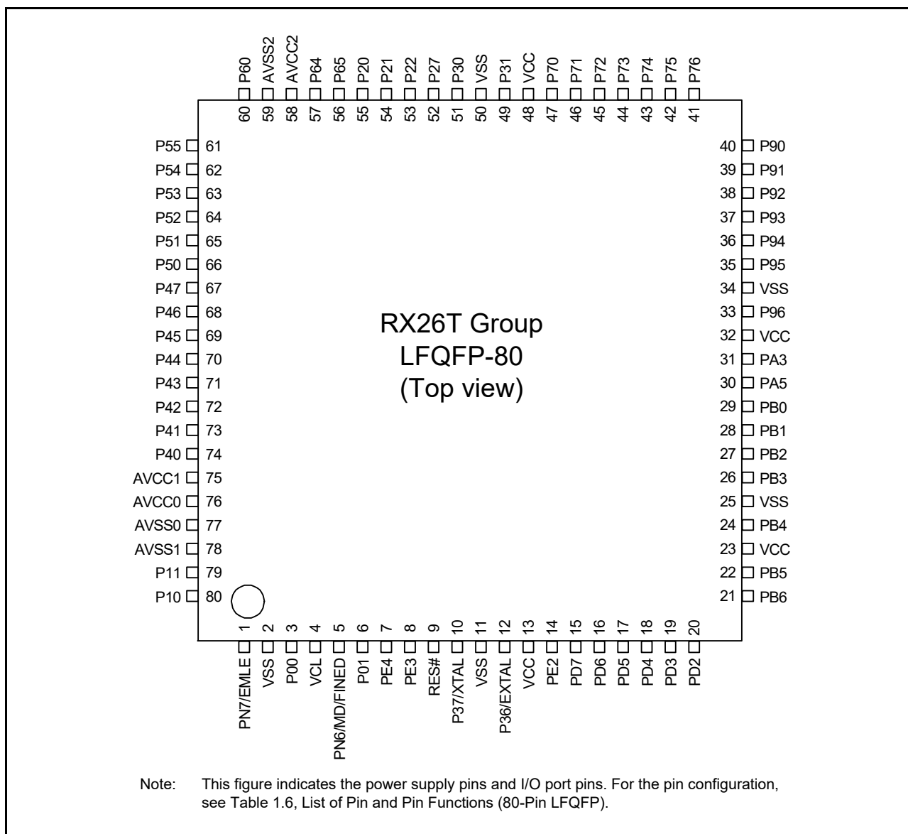
Figure 1.5 Pin Assignment (80-pin LFQFP)
