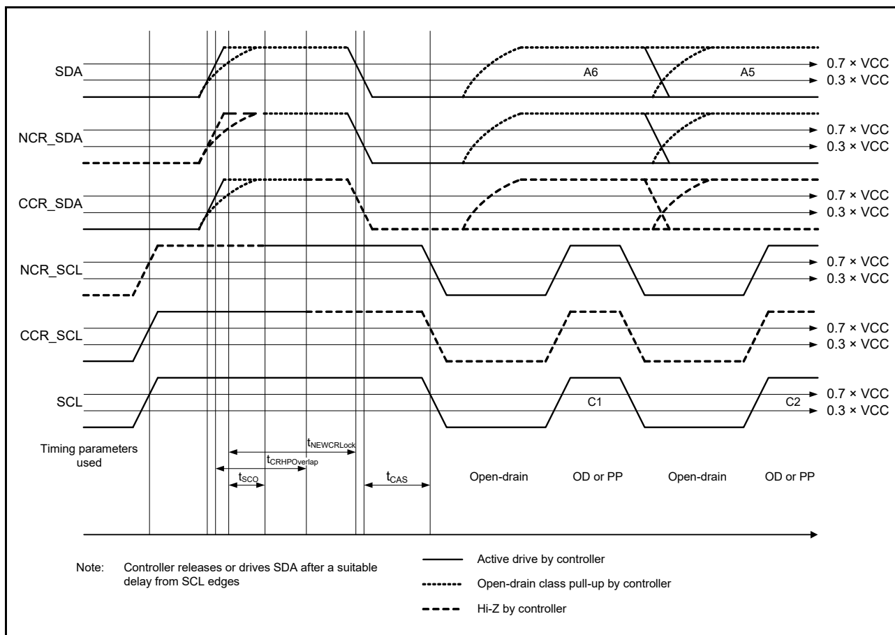
Figure 2.71 RI3C Output Timing
