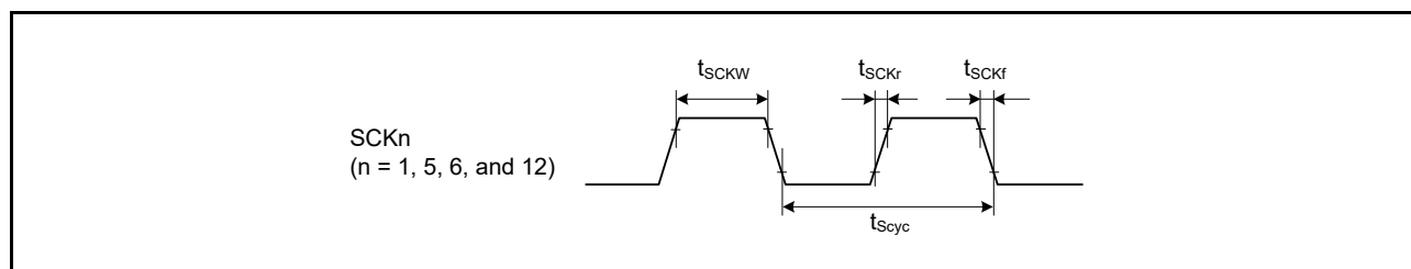
Figure 2.36 SCK Clock Input Timing
