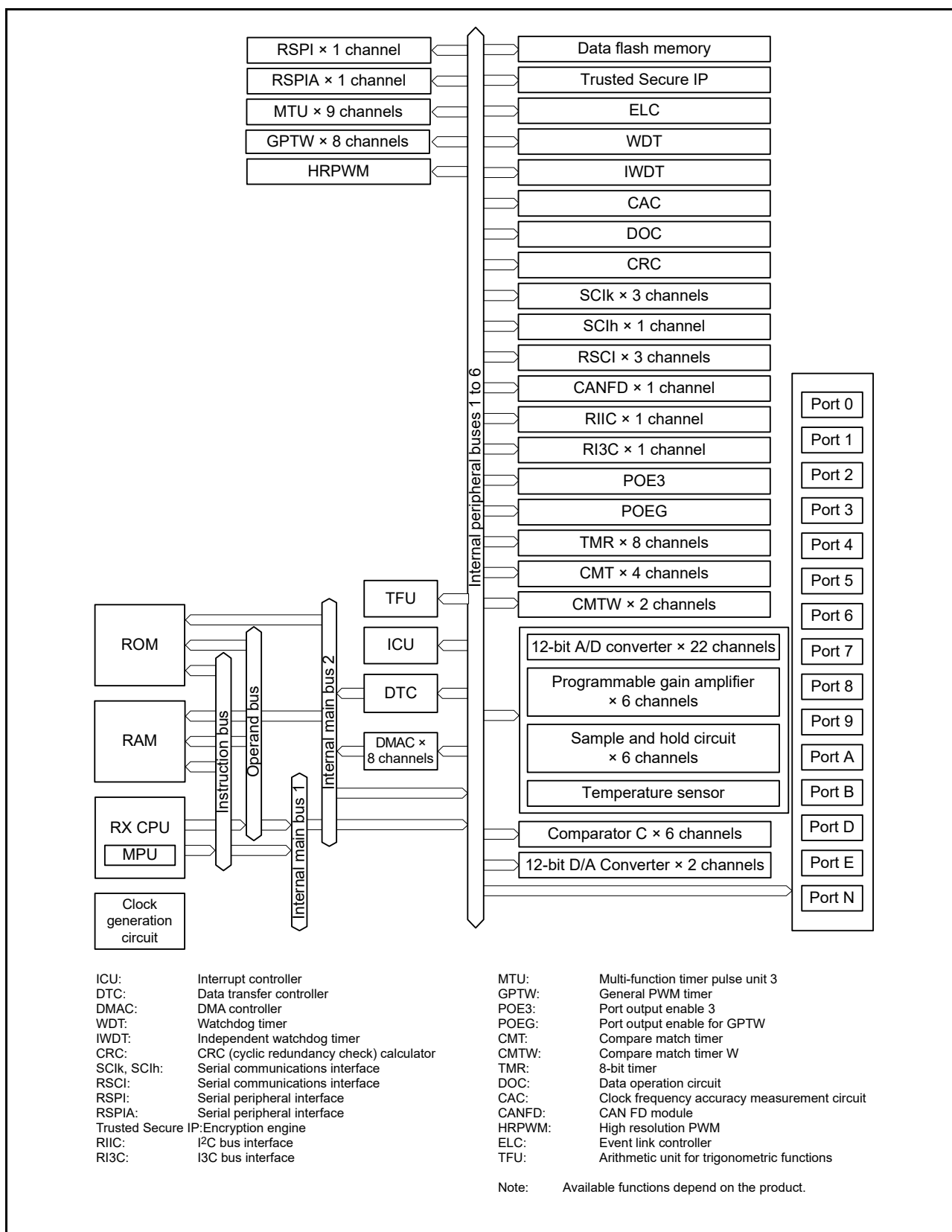
Figure 1.2 Block Diagram (Products with 64 Kbytes of RAM)
