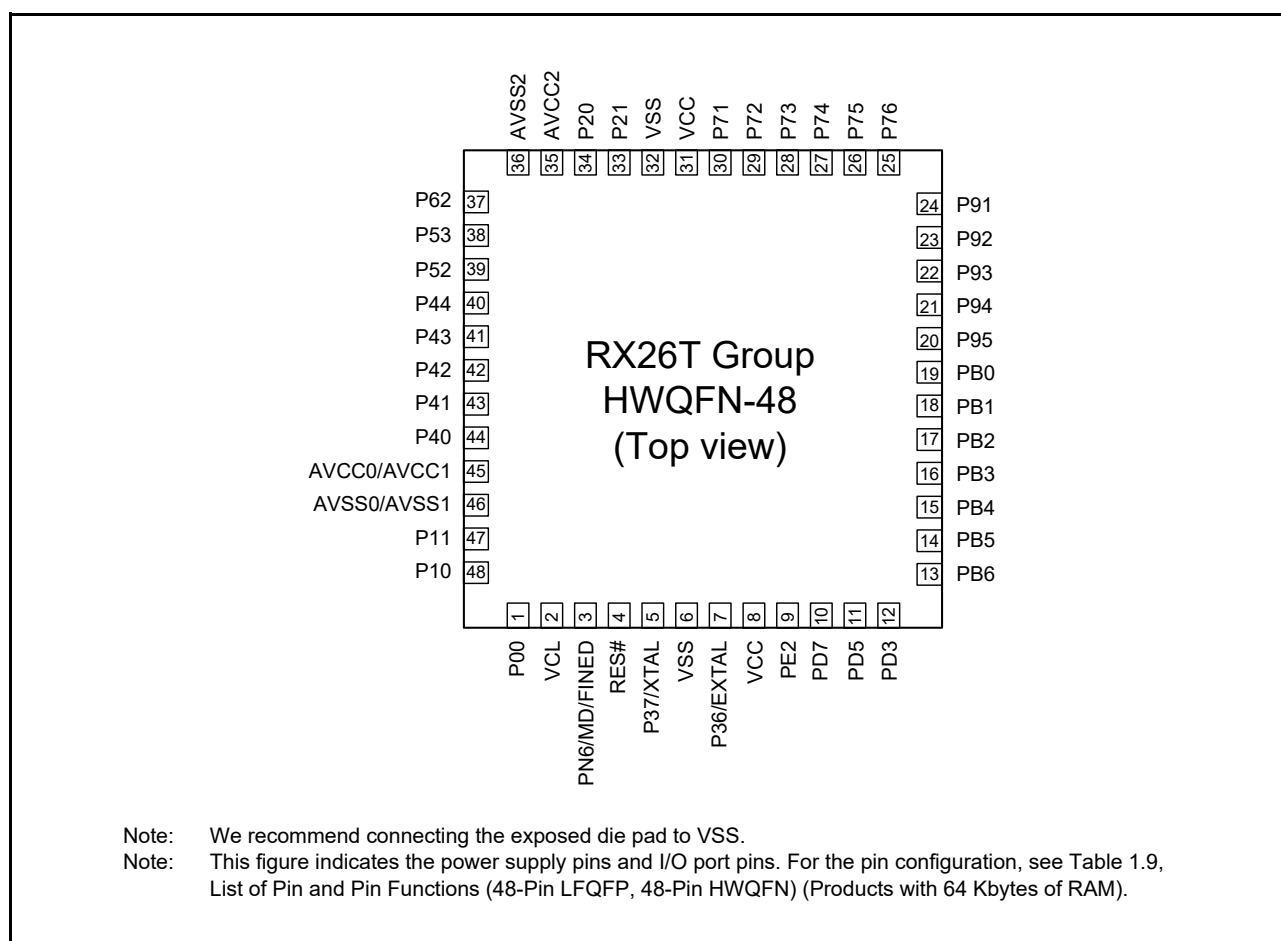
Figure 1.11 Pin Assignment (48-pin HWQFN)
