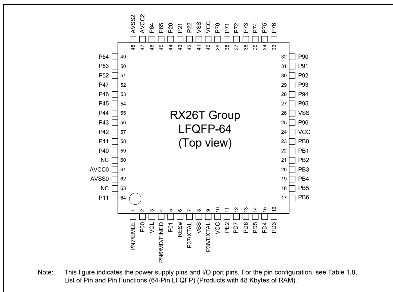
Figure 1.7 Pin Assignment (64-pin LFQFP) (Products with 48 Kbytes of RAM)
