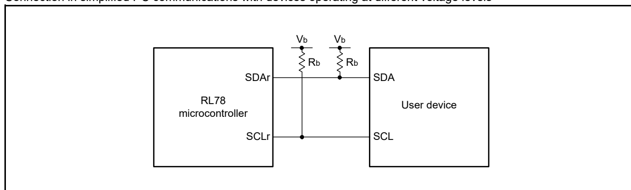
Connection in simplified I 2 C communications with devices operating at different voltage levels
