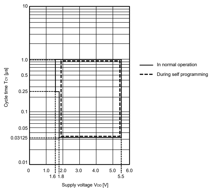
TCY vs VDD (HS (high-speed main) mode) prefetch OFF
