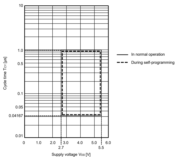
TCY vs VDD (LS (low-speed main) mode)
