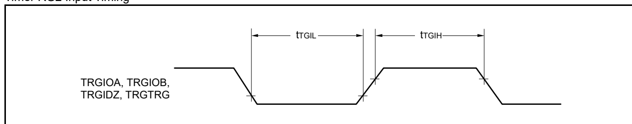
Timer RG2 Input Timing
