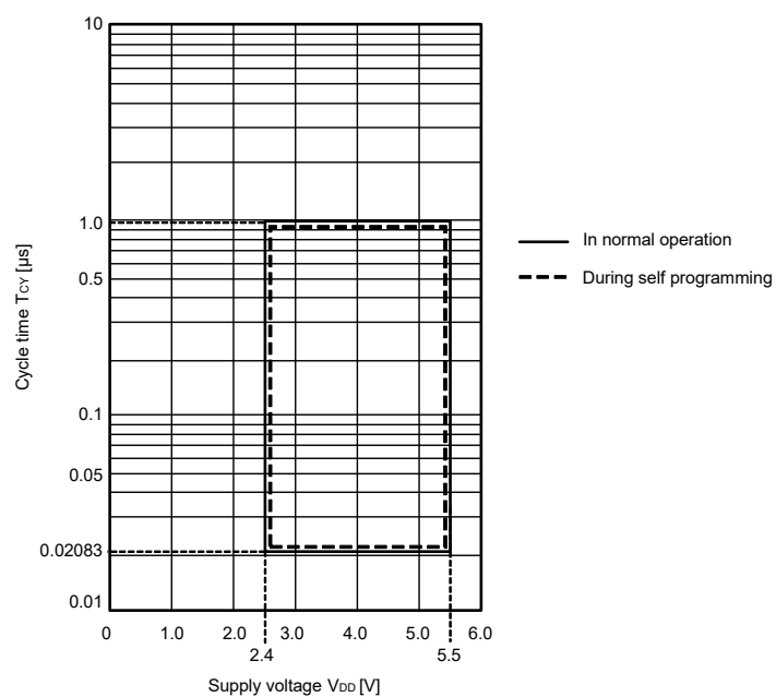
TCY vs VDD (HS (high-speed main) mode) prefetch ON
