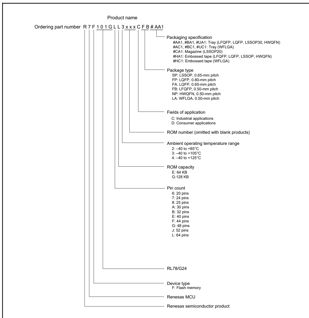
<R> Figure 1 - 1 Part Number, Memory Size, and Package of RL78/G24
