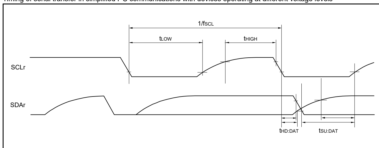
Timing of serial transfer in simplified I 2 C communications with devices operating at different voltage levels
