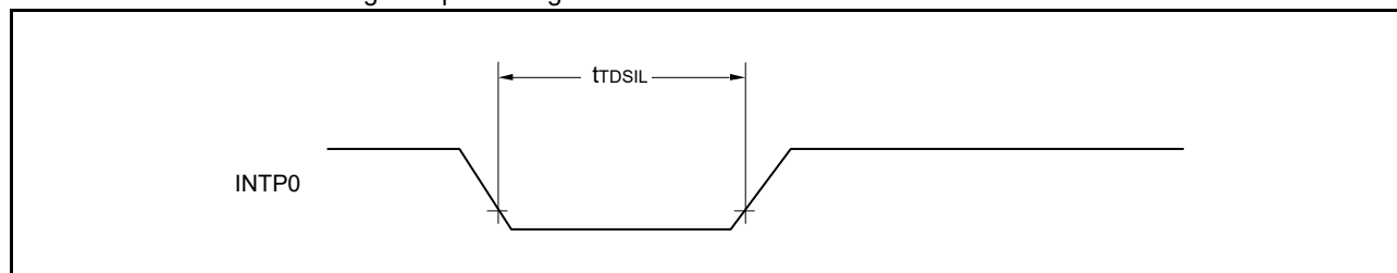
Timer RD2 Forcible Shut-off Signal Input Timing
