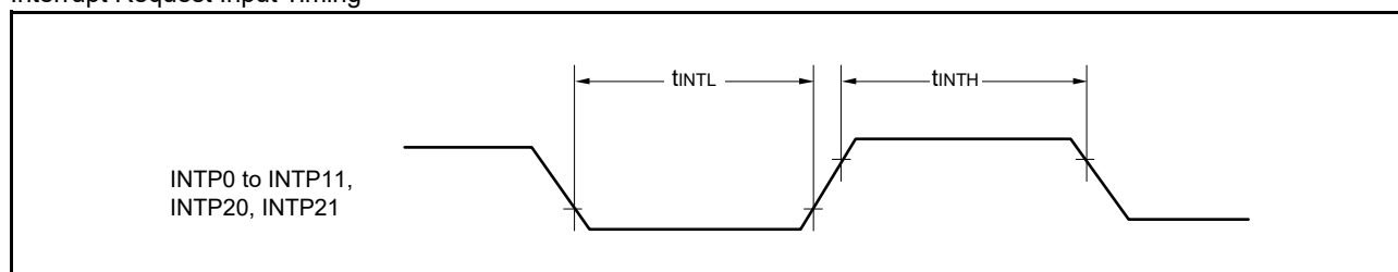
Interrupt Request Input Timing
