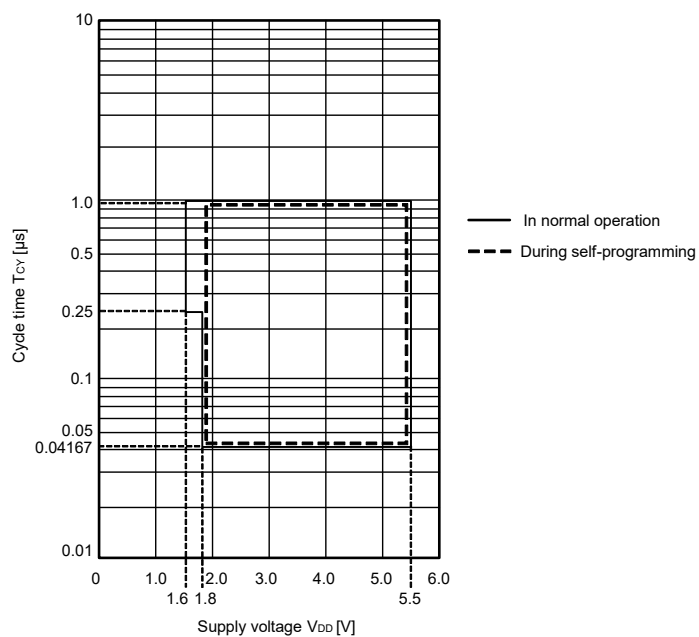
TCY vs VDD (LS (low-speed main) mode)
