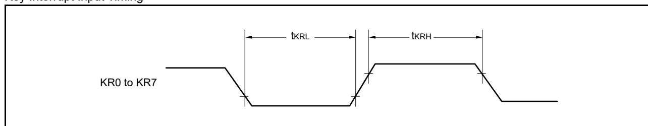
Key Interrupt Input Timing
