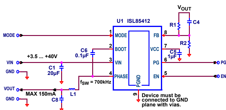
FIGURE 1. TYPICAL APPLICATION
