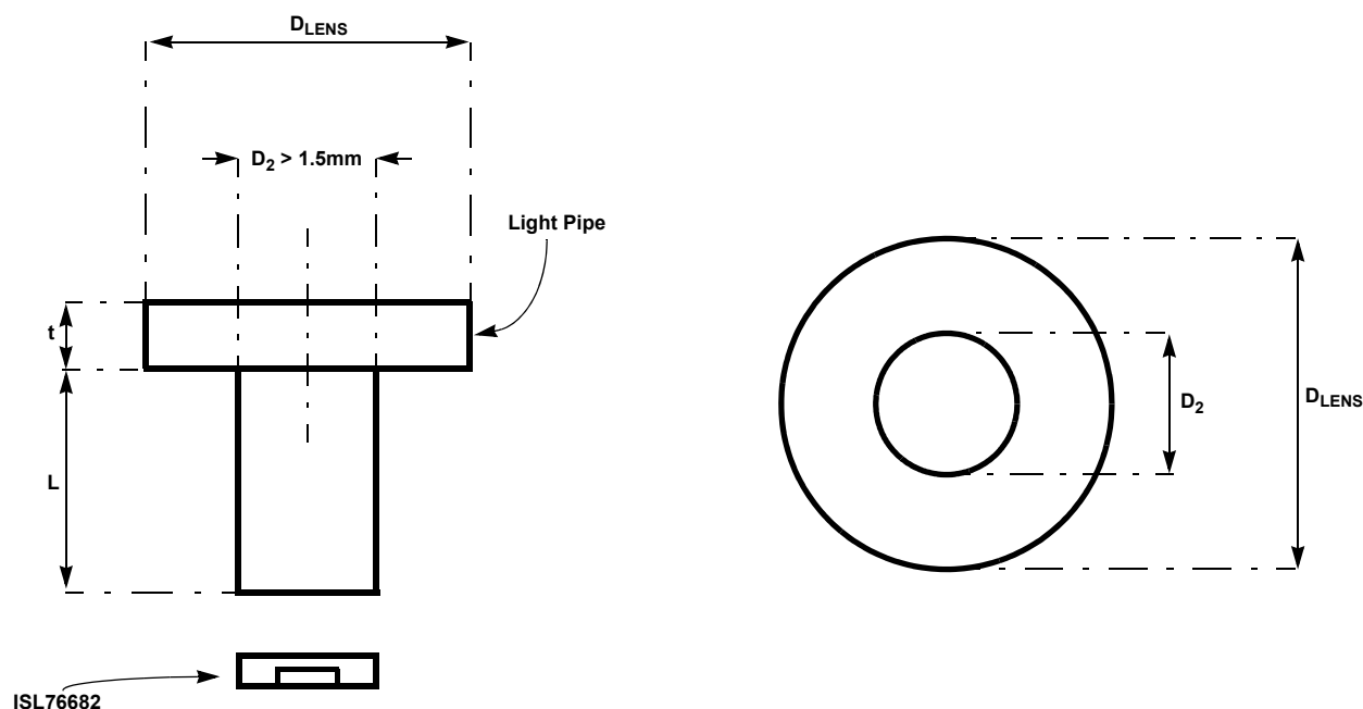
Figure 13. Window with Light Guide/Pipe
