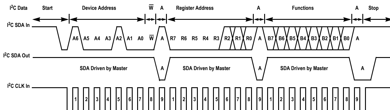
Figure 10. I 2 C Write Timing Diagram Sample
