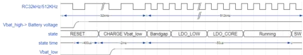
Figure 12. Power-up (Buck)
