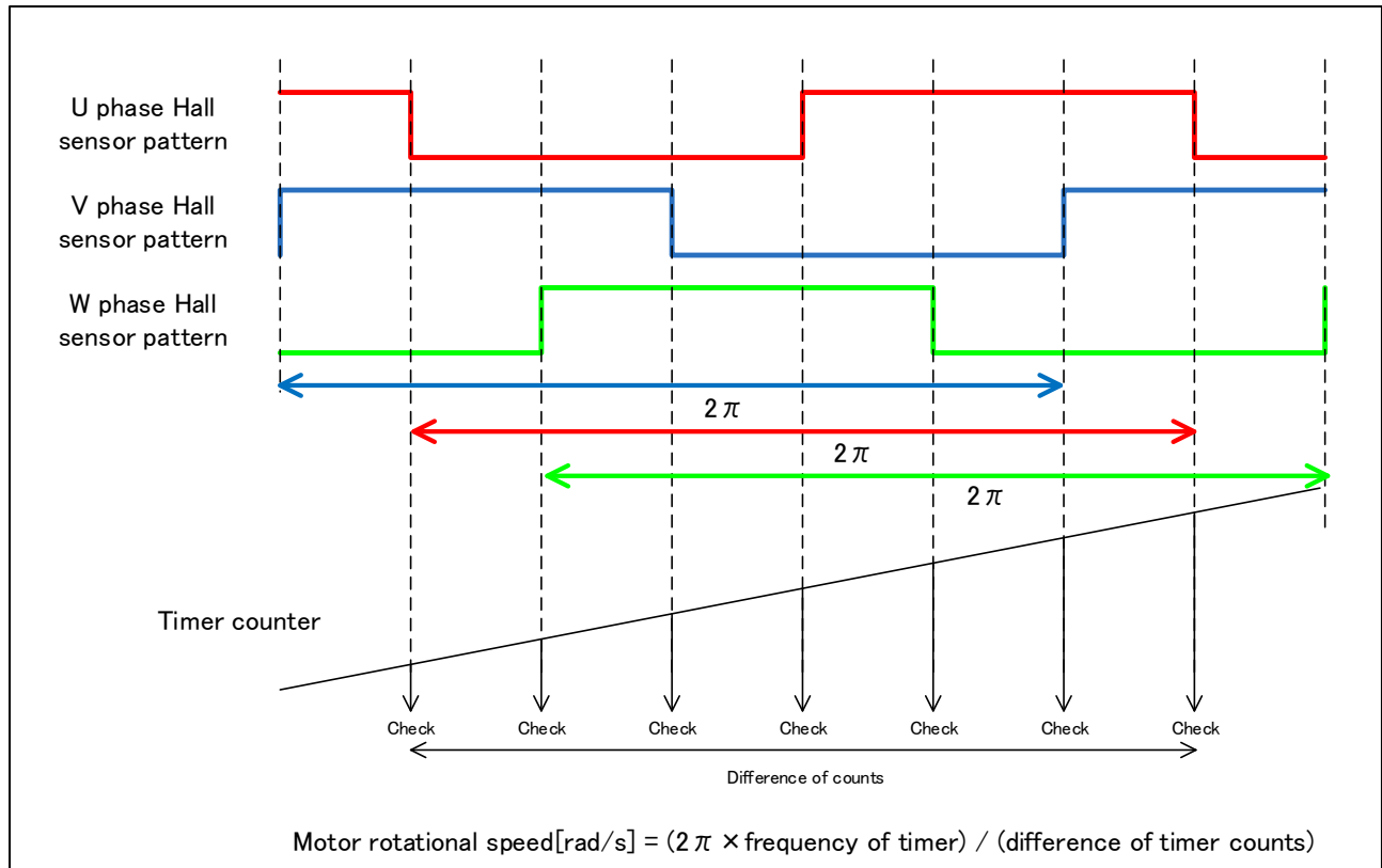
Figure 3-1 Method of Calculation for the Rotational Speed
