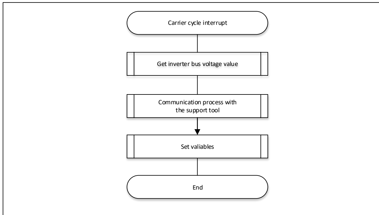
Figure 3-8 50[μs] Cycle Interrupt Handling (120-degree Control using Hall sensors)
