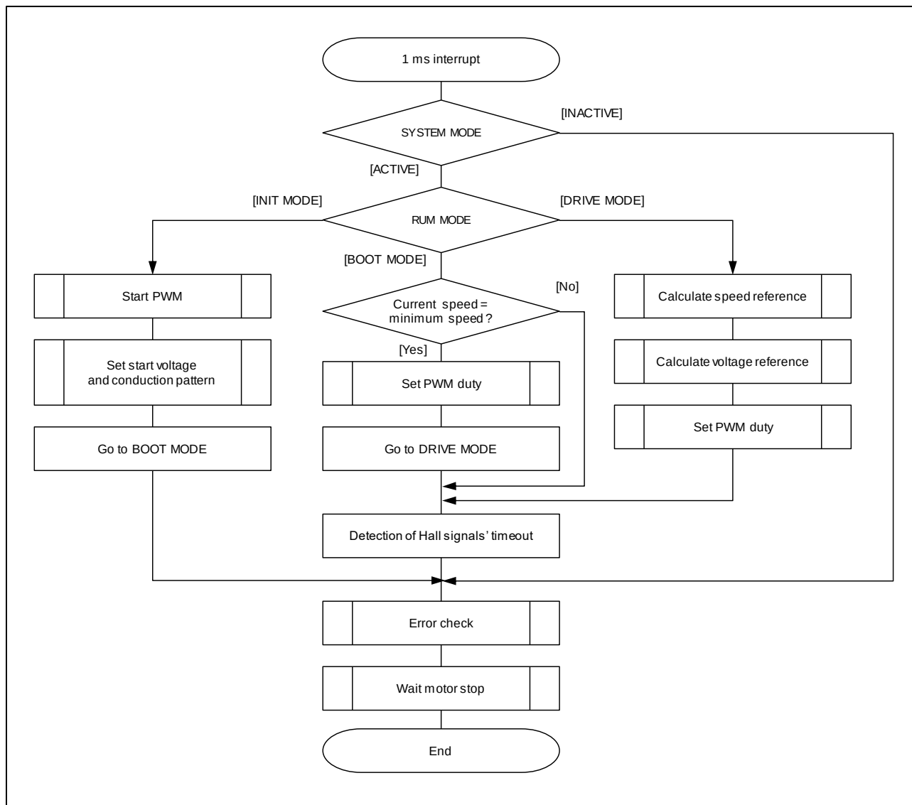
Figure 3-9 1 [ms] Interrupt Handling
