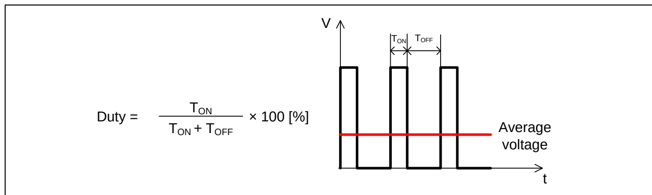
Figure 3-2 PWM Control
