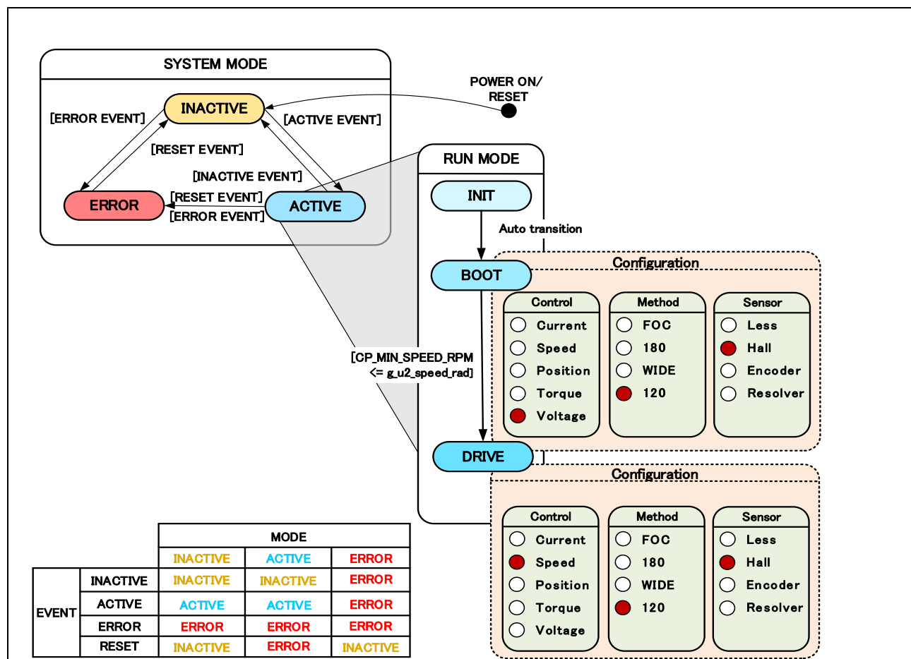
Figure 3-5 State Transition Diagram of 120-degree Conducting Control using Hall sensors Software
