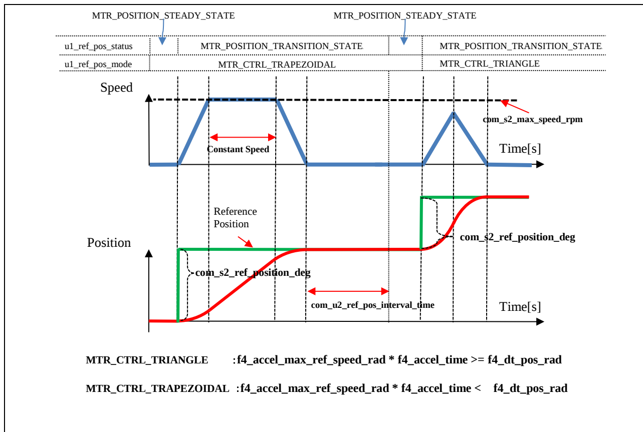
Figure 3-1 Position Profile Generation
