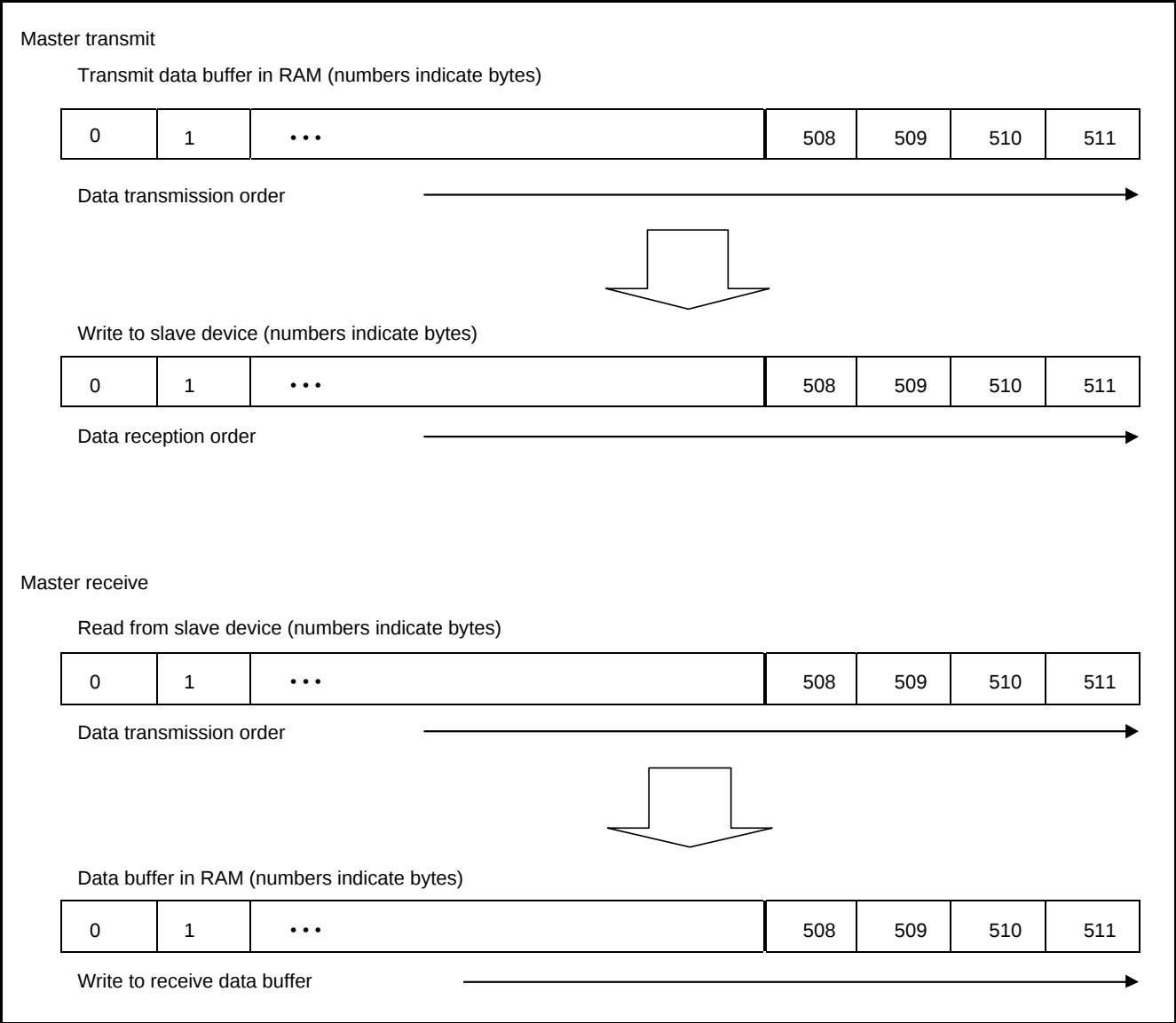
Figure 6.18 Storage of Transfer Data
