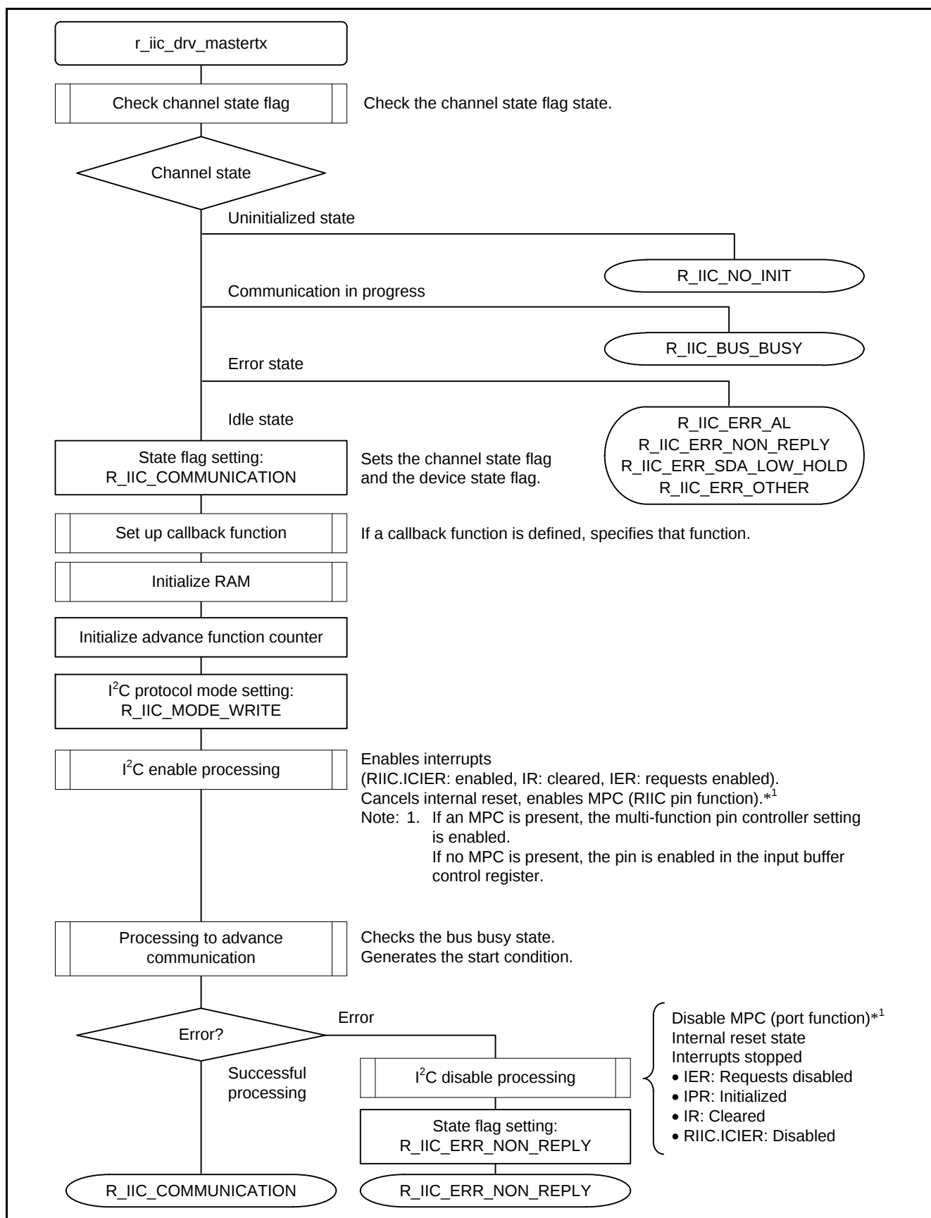
Figure 6.25 Master Transmission Start Function Overview Flowchart
