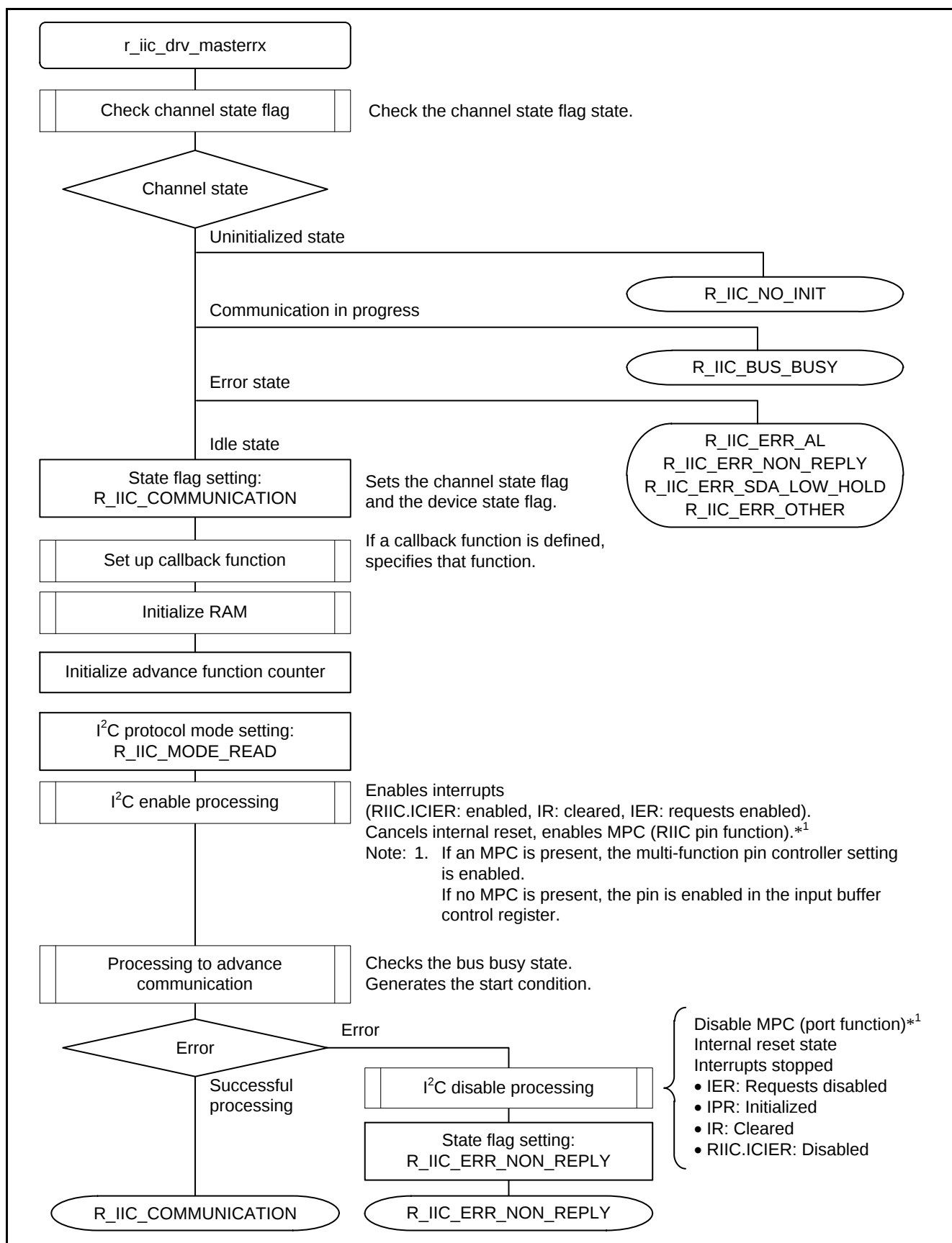
Figure 6.26 Master Reception Start Function Overview Flowchart
