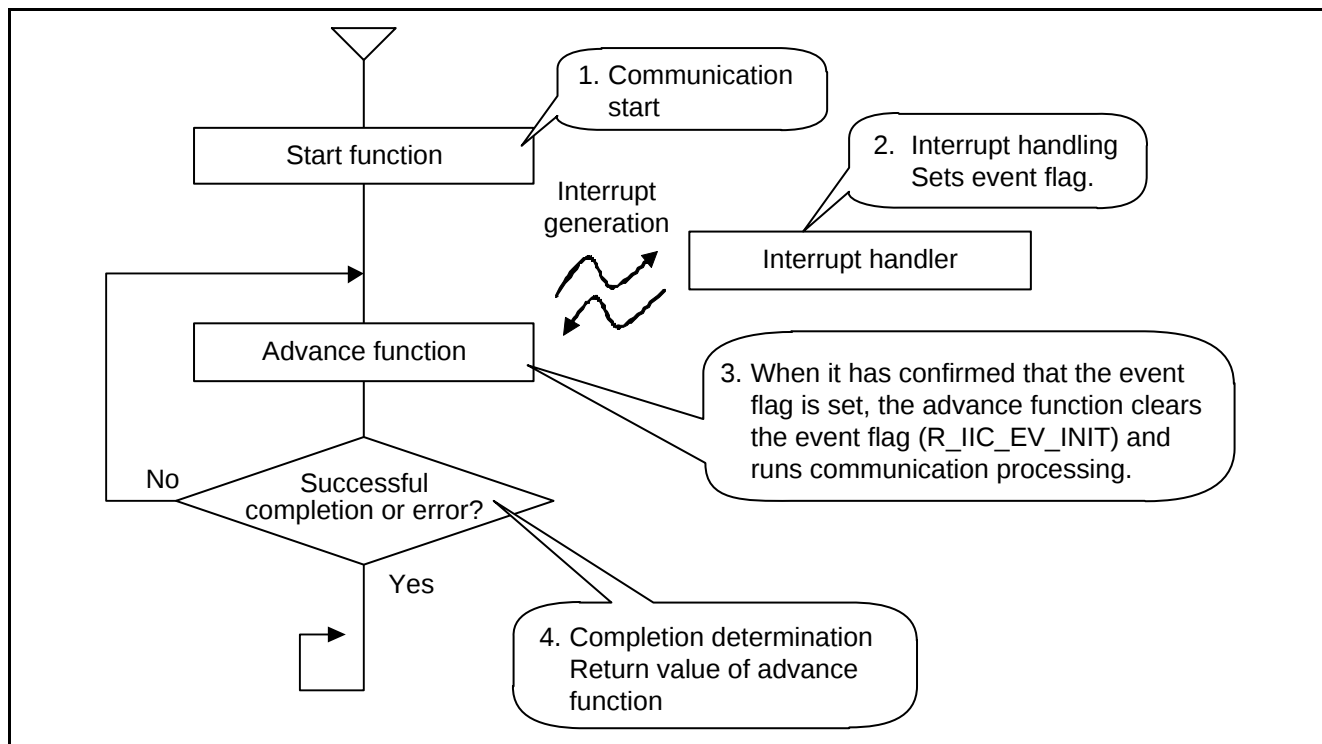
Figure 6.9 Software Operation Example: Calling the Advance Function from the Main Processing Routine
