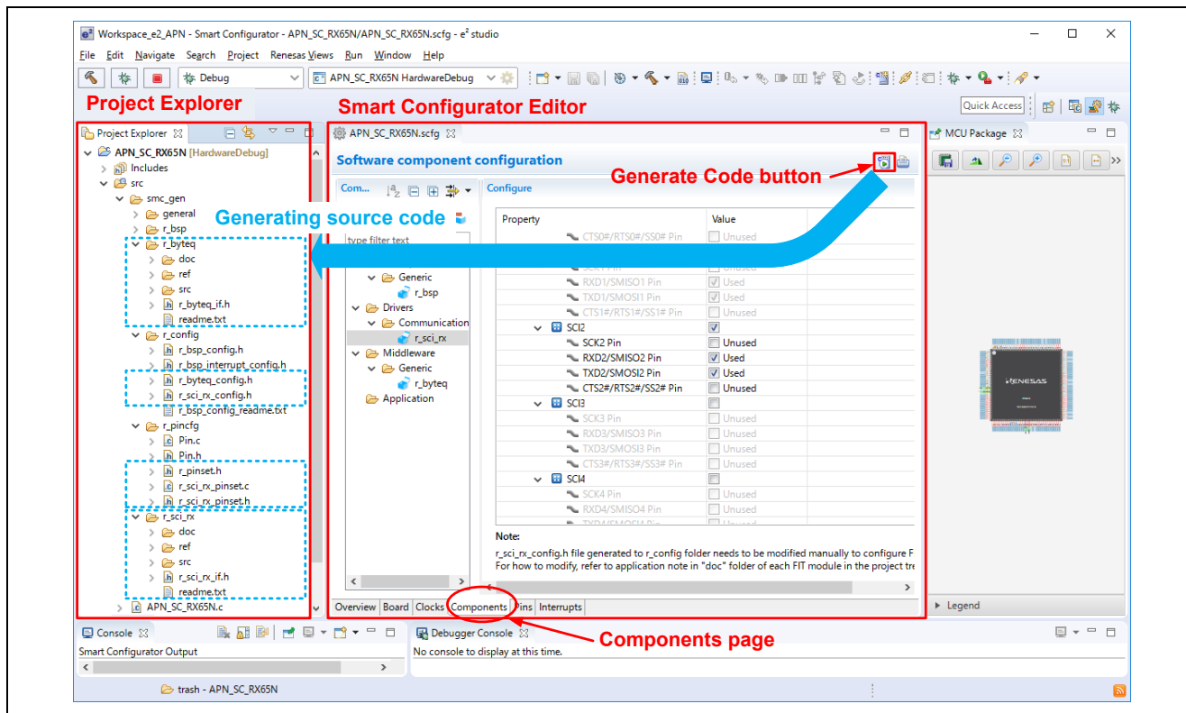
Figure 3.6 Generating the Source Code
