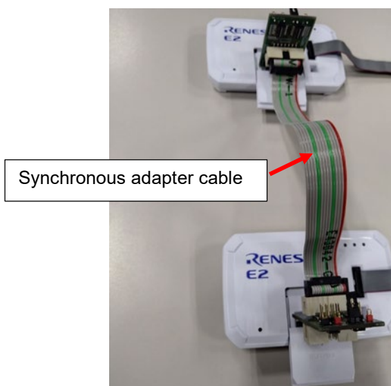
Figure 3-7 Connection of the Synchronous Adapter Cable (Case of Connecting Two E2 Emulators)
