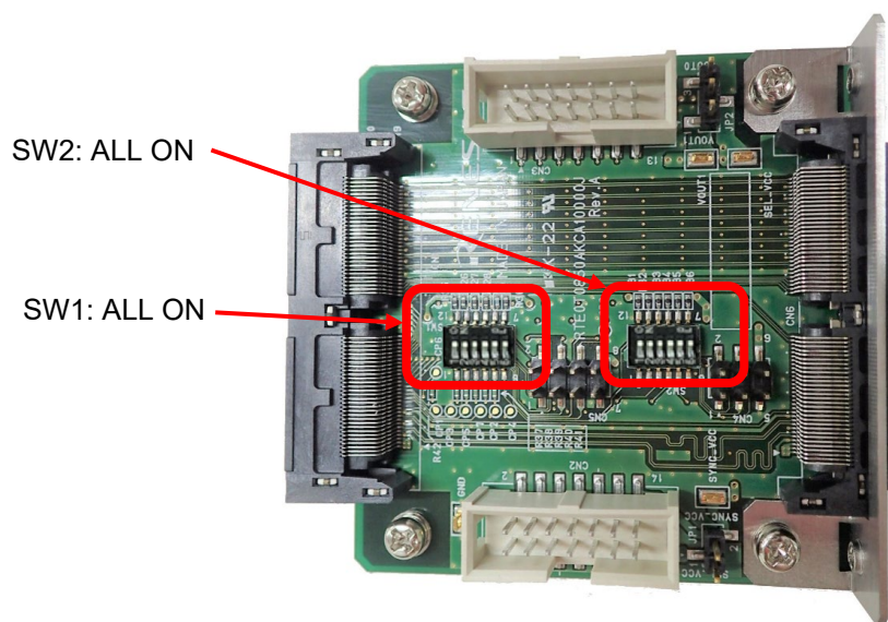
Figure 3-2 Configuration of the Synchronous Adapter for the IE850A as the First Emulator
