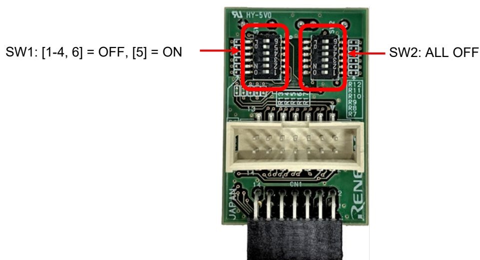
Figure 3-3 Configuration of the Synchronous Adapter for the E2 Emulator as the Second or a Subsequent Emulator
