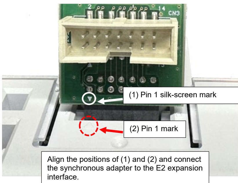
Figure 3-5 Connecting a Synchronous Adapter to the E2 Expansion Interface
