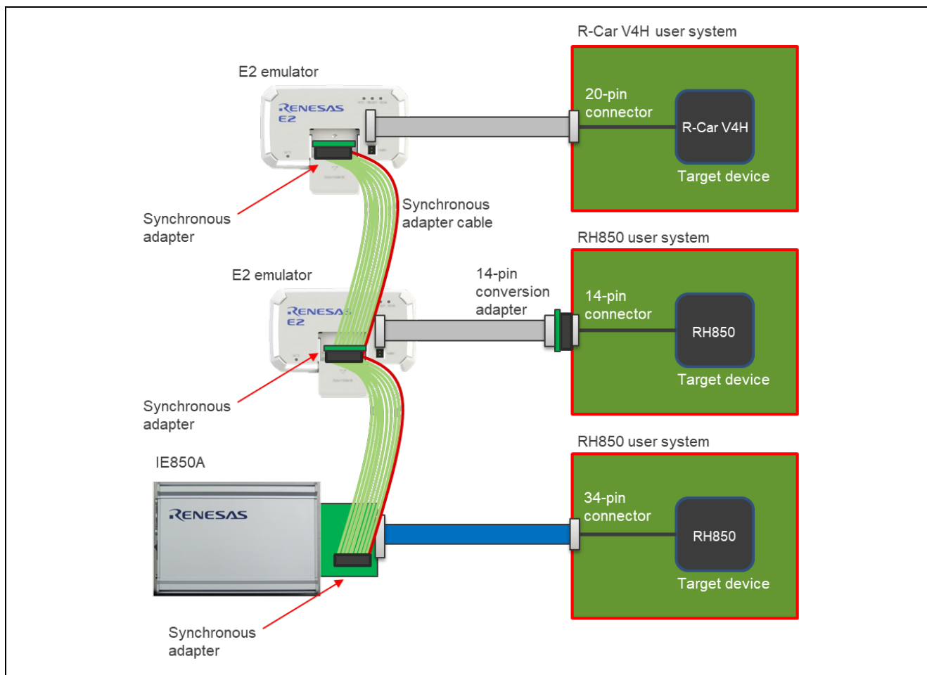
Figure 4-3 Example of Connection between the Emulators and User Systems with R-Car V4H and RH850 Devices Mounted
