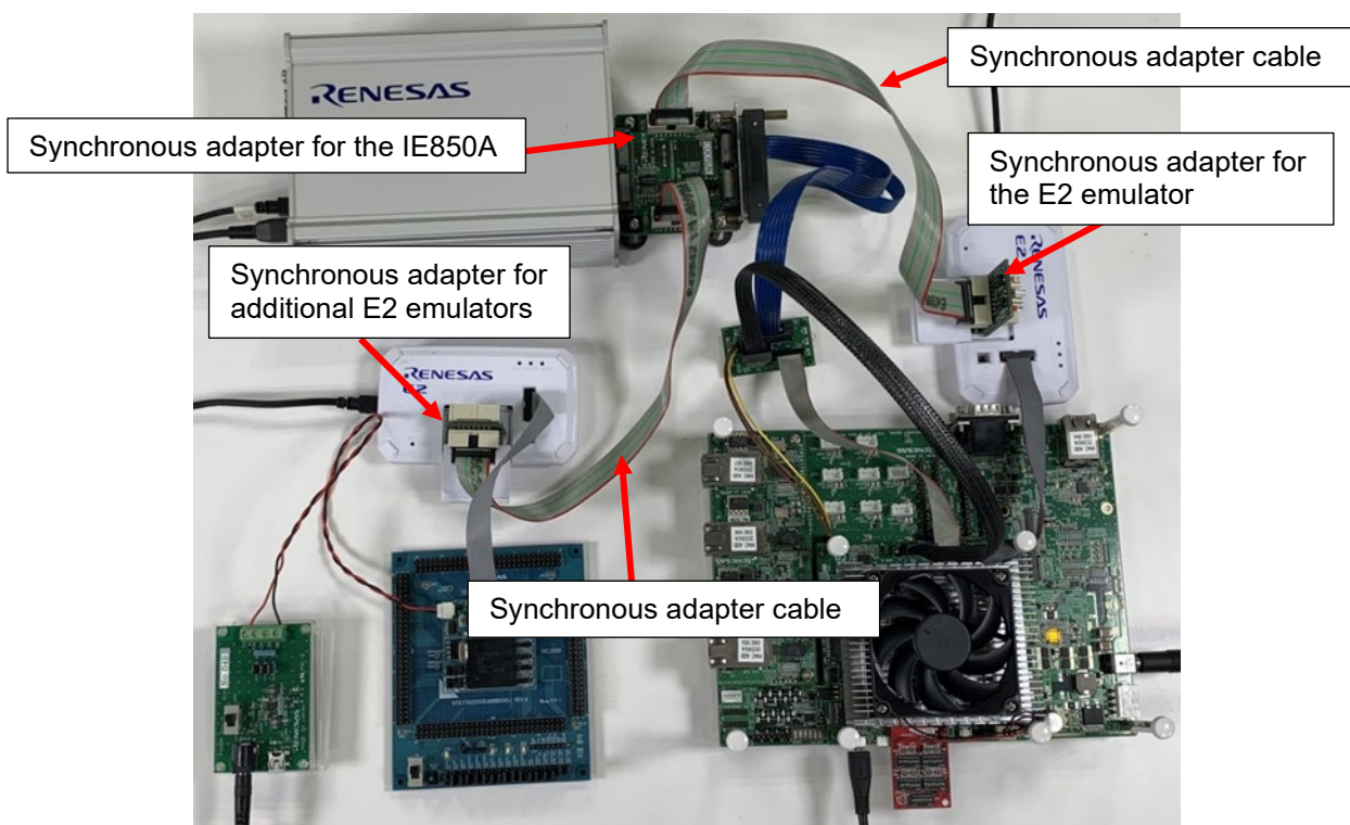
Figure 3-7 Connection of the Synchronous Adapter Cable (Case of Connecting Two E2 Emulators)
